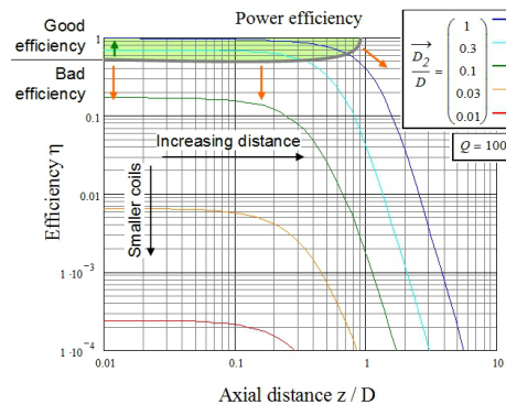
Figure 2 Power efficiency for an inductive power transfer system consisting of loop inductors in dependence on their axial distance z with size ratio as parameter. Calculated for a quality factor of Q = 100
