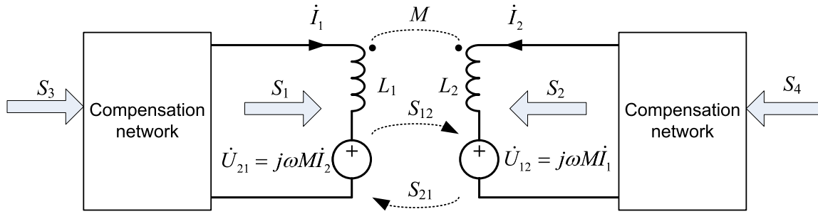
Fig. 2. General two-coil WPT system.
