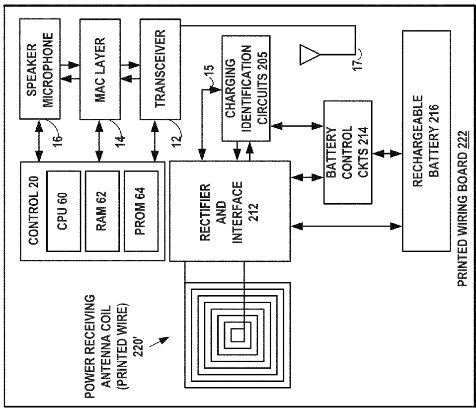
FIG. 2C SMALL RECHARGEABLE DEVICE 200
