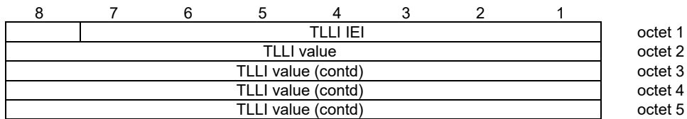
Figure 10.5.2.41a.1: TLLI information element
