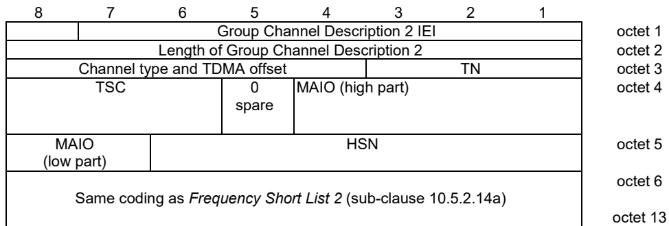
Figure 10.5.2.14f.1: Group Channel Description 2 information element
