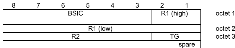
Figure 9.1.30b.1: COMPACT Frame synchronization information element
