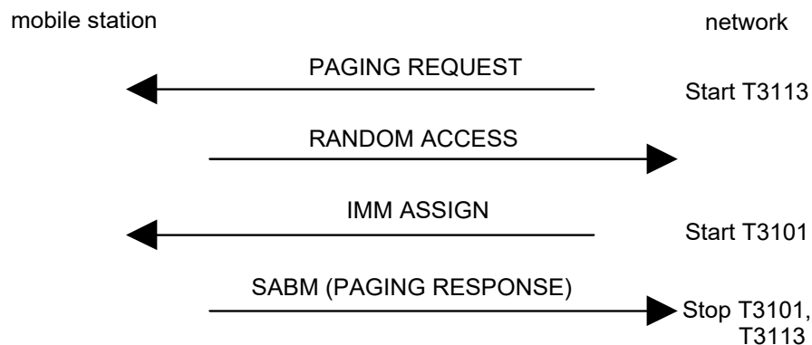
Figure 3.3.2.3.1: Paging sequence
