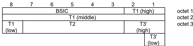
Figure 9.1.30a.1: Frame synchronization information element
