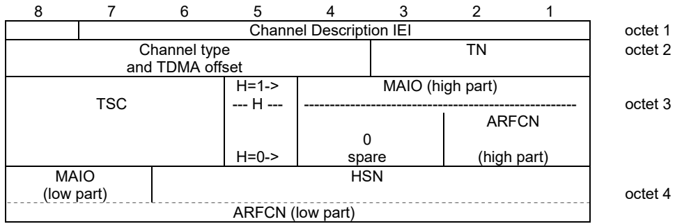
Figure 10.5.2.5a.1: Channel Description 2 information element
