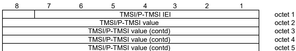
Figure 10.5.2.42.1: TMSI/P-TMSI information element
