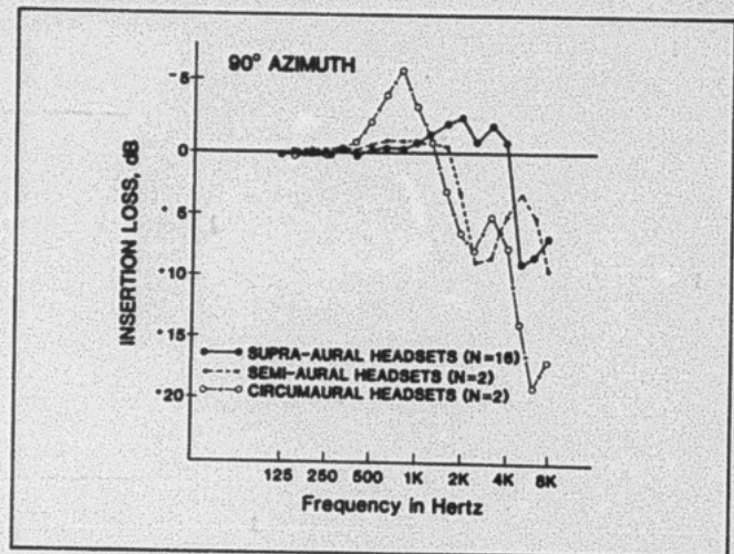
Figure 7. Insertion loss characteristics of personal radio headsets at 90° azimuth.
