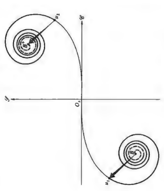
Figure 10.60 The Cornu spiral as applied to a narrow obstacle.
