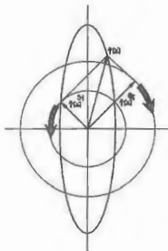
Figure 8.8 Elliptical light as the superposition of an \mathcal{E} - and \mathcal{E} -state.
