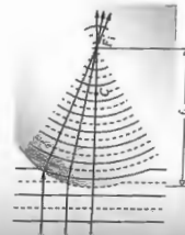
Figure 5.9 The reshaping of plane into spherical waves at a spherical interface— F_i is the image focus.
