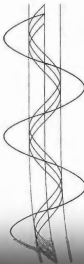
Figure 7.5 The superposition of three harmonic waves yields a harmonic wave of the same frequency.
