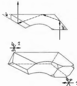
Figure 5.67 The Leman-Springer prism.
