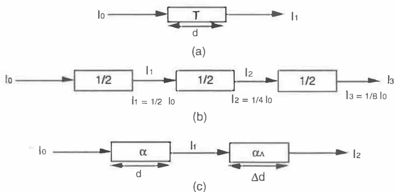
Figure 9.1. A block diagram illustrating the transmittance of light through a block model of the components of a finger. (a) Incident light having an intensity of I_0 impinges upon an absorptive medium with a characteristic transmittance factor T . (b) The effect of a medium divided into n identical components of unit thickness and same transmittance factor T on incident light intensity I_0 . (c) For a finger model, the baseline component of the unchanging absorptive elements and the pulsating component of the changing absorptive portion are represented (Cheung et al 1989).
