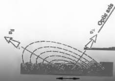
Figure 8.22 Wavelets within calcite.
