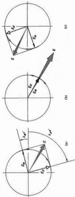
Figure 8.50 The superposition of \mathcal{D} - and \mathcal{L} -states at z = z' (k_y > k_x) .
