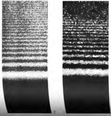
The fringe pattern for a half-screen formed with light. (Francis Weston Davis, ©1949, Addison-Wesley Reading, MA.) (b) Fresnel electron diffraction of a half plane (MGO crystal)—electrons behave like photons. (Photo courtesy of Physik, edited by S. Flugge, Springer-Verlag, Heidelberg.)
