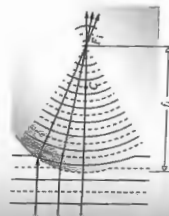
Figure 5.9 The reshaping of plane into spherical waves at a spherical interface—the image focus.
