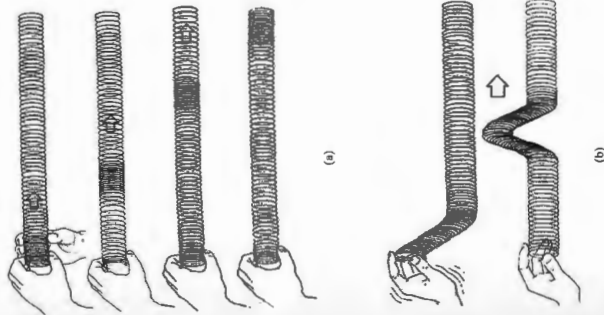
Figure 2.1 (a) A longitudinal wave in a spring. (b) A transverse wave in a spring.
