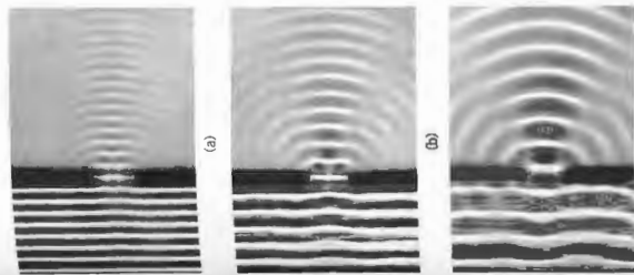
Figure 10.3 Diffraction through an aperture with varying \lambda , as seen in a ripple tank. (a) \lambda > \Delta_{\text{max}} ; (b) \lambda \approx \Delta_{\text{max}} ; (c) \lambda < \Delta_{\text{max}} . (Photo courtesy PSSC Physics, D. C. Heath, Boston, 1960.)
