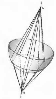
Figure 5.7 Rays incident at the same angle.
