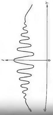
Figure 12.10 A finite bandwidth results in a decreasing value of \bar{I} with increasing y .
