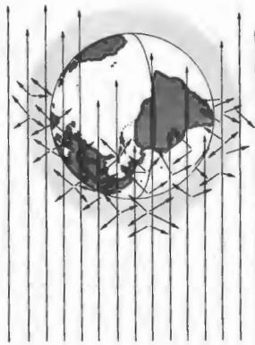
Figure 8.29 Scattering of sky light.
