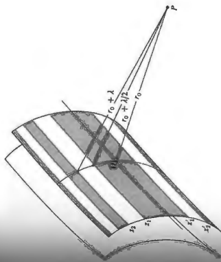
Figure 10.52 Cylindrical wavefront zones.
