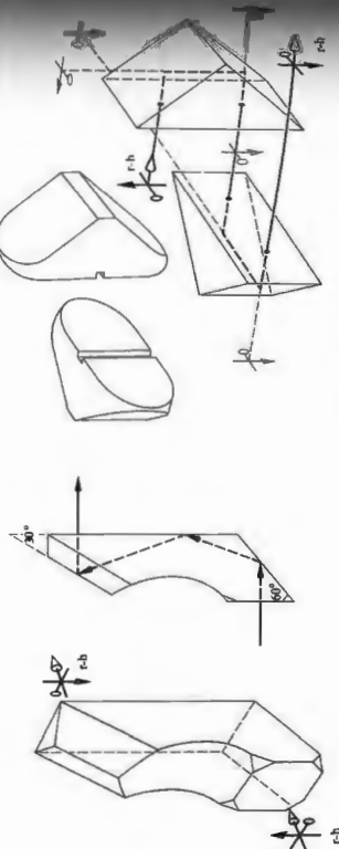
Figure 5.68 The double Porro prism.
