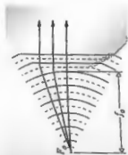
Figure 5.8 Plane waves propagating beyond a spherical interface—image focus.
