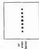
Diffraction pattern
