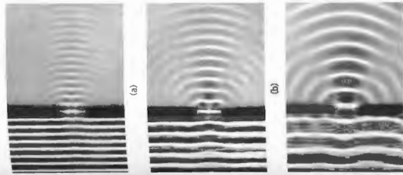
Figure 10.3 Diffraction through an aperture with varying \lambda , as seen in a ripple tank. (a) \lambda > \lambda_{\max} ; (b) \lambda < \lambda_{\max} ; (c) \lambda = \lambda_{\max} . (Photo courtesy PSSC Physics, D. C. Heath, Boston, 1960.)
