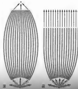
Figure 5.78 A bundle of multichannel threads used to (a) focus or collimate X-rays from a point source.
