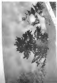
Looking down into a puddle (that's melting snow on the right) we see a reflection of the surrounding trees. At normal incidence we see reflections that are 2% of the light. As the viewing angle increases here its about 40% of the percentage increases. (Photo by E.N.)
