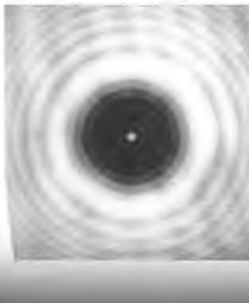
Figure 10.43: A photograph of a 1/8-inch diameter ball bearing. The bearing was glued to a microscope slide and illuminated with a He-Ne laser beam. There are some faint extraneous nonconcentric fringes arising from both the microscope slide and a lens in the beam. (Photo by E.H.)
