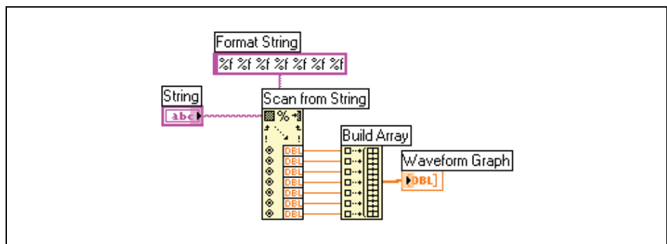
Figure 9-2. Converting a String to Numerics
