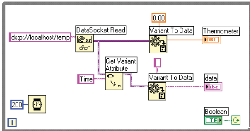
Figure 17-4. Converting Live Variant Data to Temperature Data
