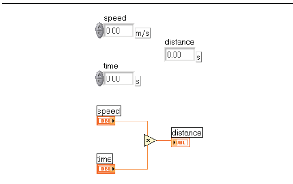
Figure 5-5. Wiring Objects with Compatible Units
