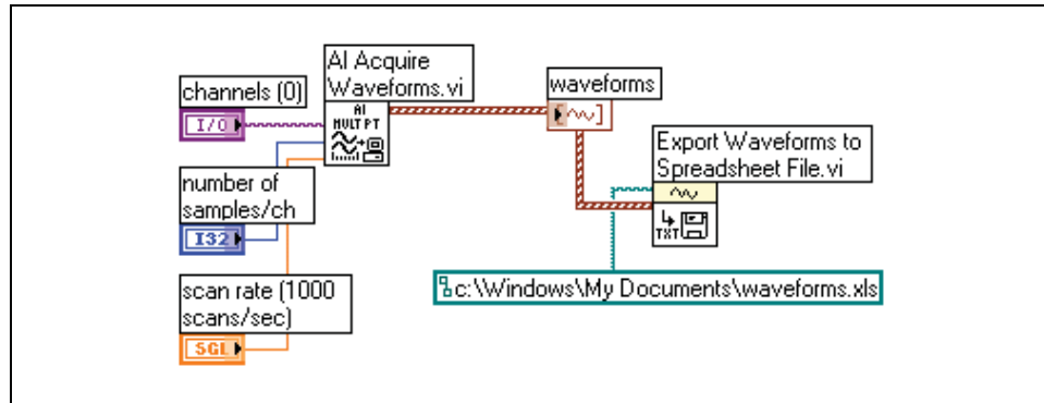
Figure 13-3. Writing Multiple Waveforms to a Spreadsheet File
