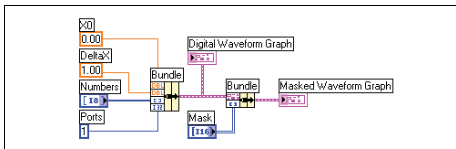
Figure D-1. Masking Digital Data
