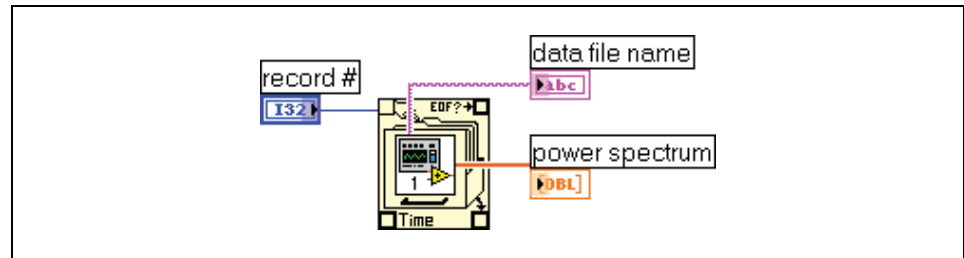
Figure 13-9. Retrieving Logged Data through SubVI Terminals
