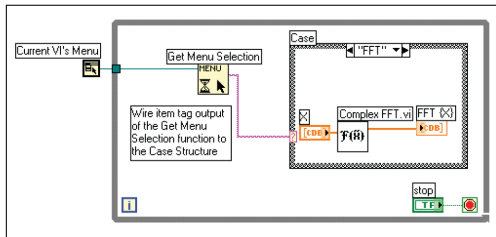
Figure 15-1. Block Diagram Using Menu Handling
