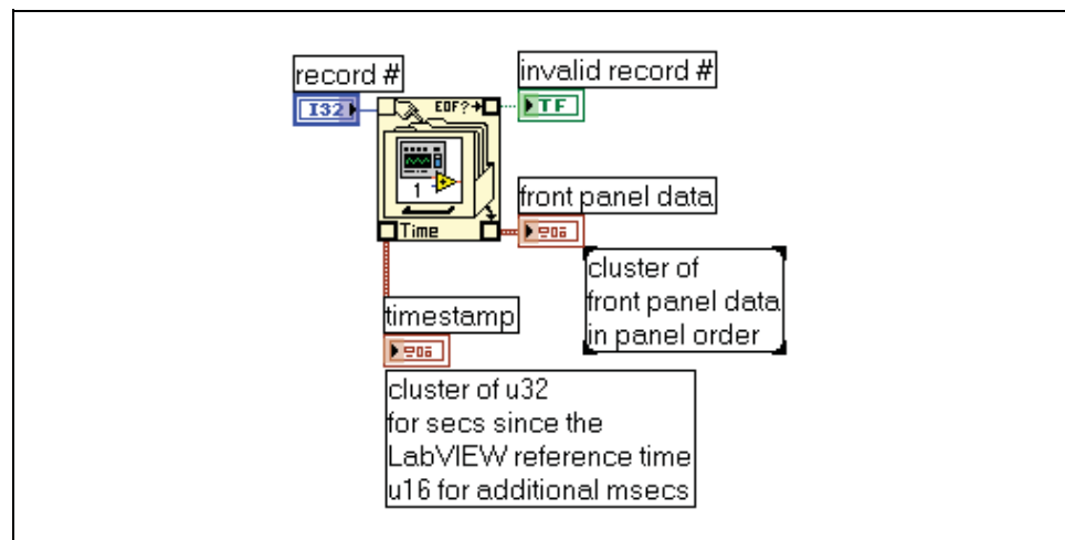
Figure 13-8. Retrieving Logged Data
