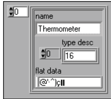
Figure 5-4. Cluster of Flattened Numeric Data
