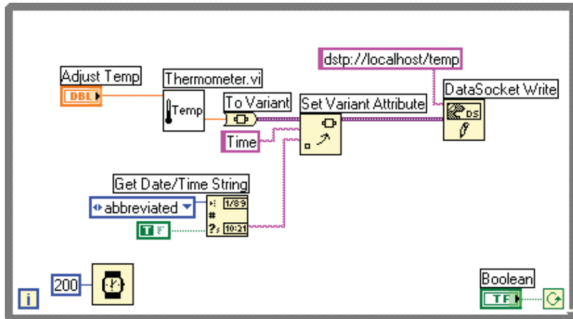
Figure 17-3. Converting Live Temperature Data to Variant Data
