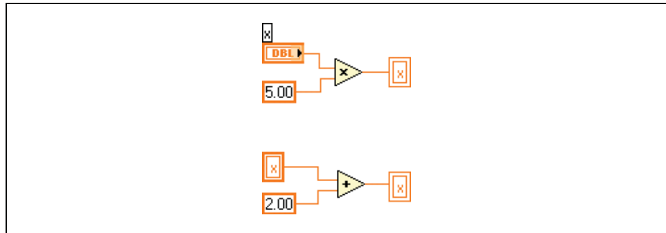
Figure 10-1. Race Condition
