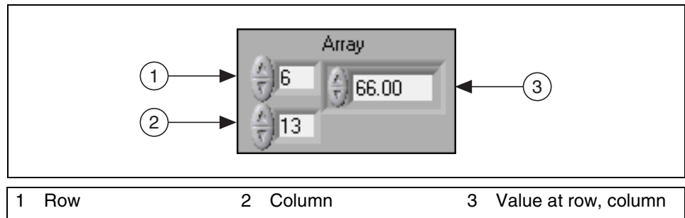
Figure 9-8. Array Control
