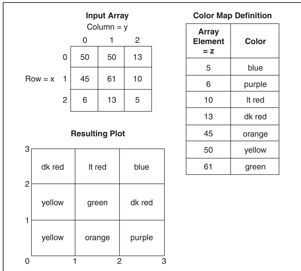
Figure 11-5. Intensity Chart Color Map
