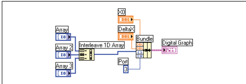
Figure 11-8. Using Interleave Function with Digital Graph
