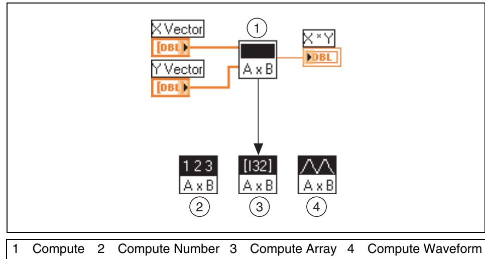
Figure 5-3. Polymorphic VI Calling a SubVI
