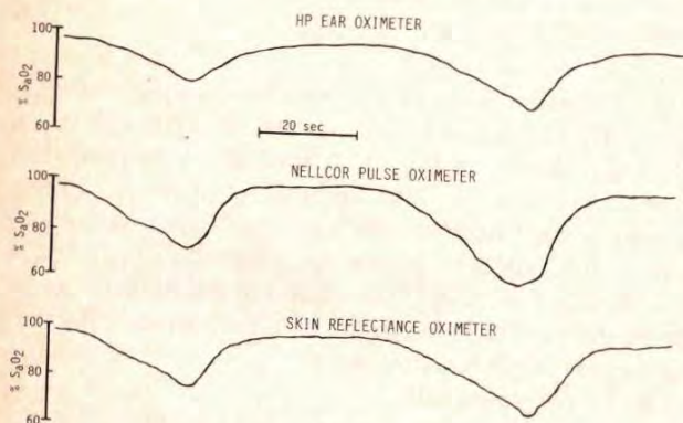
Fig. 10. Simultaneous recordings of SaO_2 from the HP ear oximeter, Nellcor pulse oximeter and the prototype reflectance pulse oximeter.
