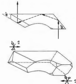
Figure 5.67 The Leman-Springer prism.
