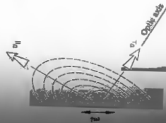
Figure 8.22 Wavelets within calcite.
