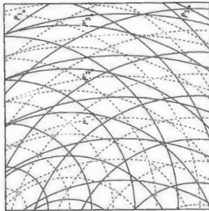
Figure 9.4 Temporal and spatial coherence. (a) Here the waves display complete temporal coherence. (b) Here there is complete spatial coherence but only partial temporal coherence.
