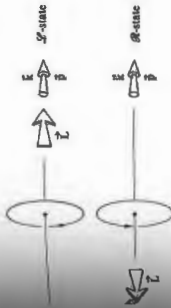
Figure 8.9 Angular momentum of a photon.
