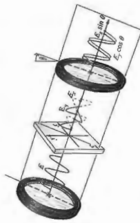
Figure 8.46 The origin of interference colors.
