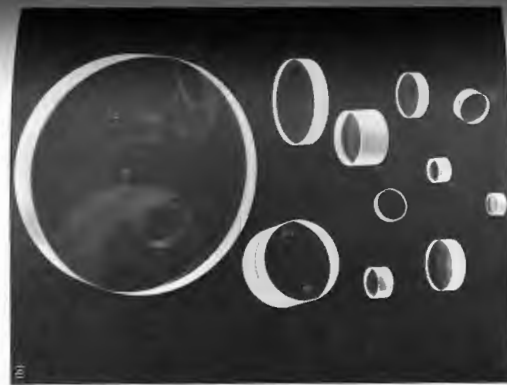
Figure 6.40 (a) Achromatic doublets. (b) Doublets and triplets courtesy Moles Grieb.
