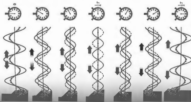
Figure 7.10 The creation of standing waves. Two waves of the same amplitude and wavelength traveling in opposite directions form a stationary disturbance that oscillates in place.
