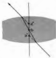
Figure 6.2 Nodal points.
