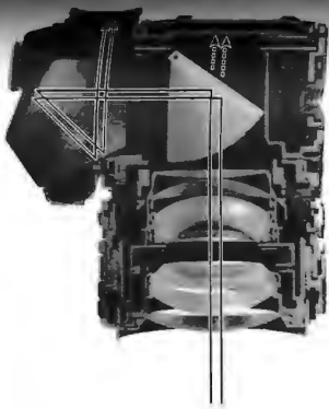
A single-lens reflex camera. Light from the lens hits the mirror and goes up to the prism and out to the eye. When the shutter is released, the mirror flips up, the light goes directly to the film, and then the mirror pops back down. (Photo by E.H.)
