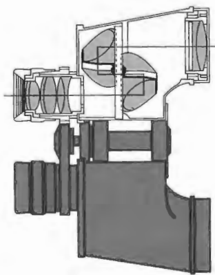
Figure 5.109 A binocular.
