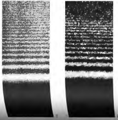
The fringe pattern for a half-screen formed with light. (Francis Weston Davis, ©1949, Addison-Wesley Reading, MA.) (b) Fresnel electron diffraction by a half plane (MgO crystal)—electrons behave like photons. (Photo courtesy of S. Flugge, Springer-Verlag, Heidelberg.)
