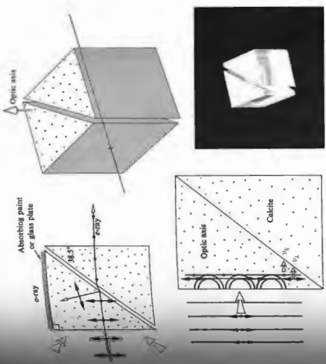
Figure 8.27 The Glan-Foucault prism. (Photo by E.H.)
