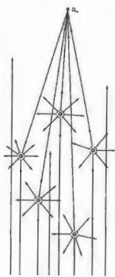
Figure 4.4 Scattering in the forward direction doesn't change the light paths very much, and the waves all arrive at P pretty much in-phase.
