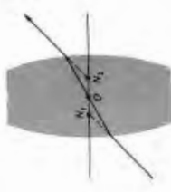
Figure 6.2 Nodal points.
