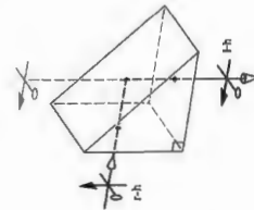
Figure 5.61 The right-angle prism.
