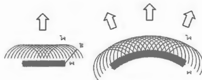
Figure 4.26 According to Huygens's Principle, a wave propagating if the wavefront were composed of an array of point sources, each emitting a spherical wave.
