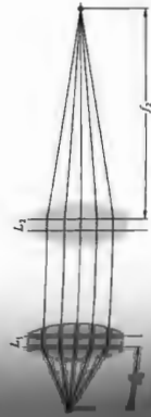
Figure 6.24 A combination of two infinite conjugate lenses yielding a coma-free image at finite conjugates.
