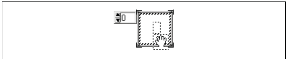
Figure 9-7. Array Shell
