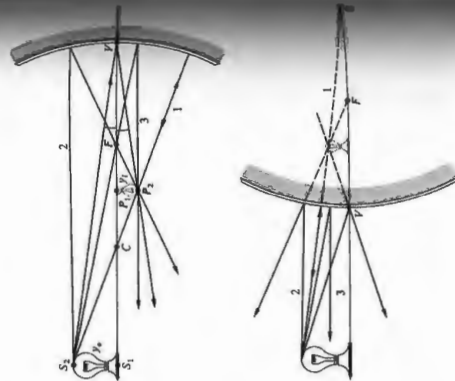
Figure 5.52 Four easy rays to draw. Ray 1 heads toward C and reflects back along itself. Ray 2 comes in parallel to the central axis and reflects toward (or away from) F . Ray 3 passes through (or heads toward) F and reflects off parallel to the axis. Ray 4 strikes point V and reflects such that \theta_i = \theta_r .
