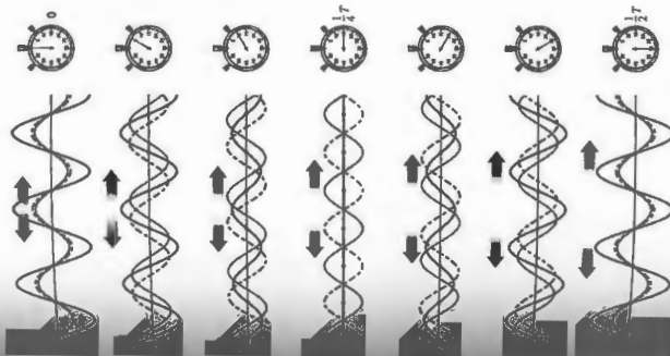
Figure 7.10 The creation of standing waves. Two waves of the same amplitude and wavelength traveling in opposite directions form a stationary wave that oscillates in place.
