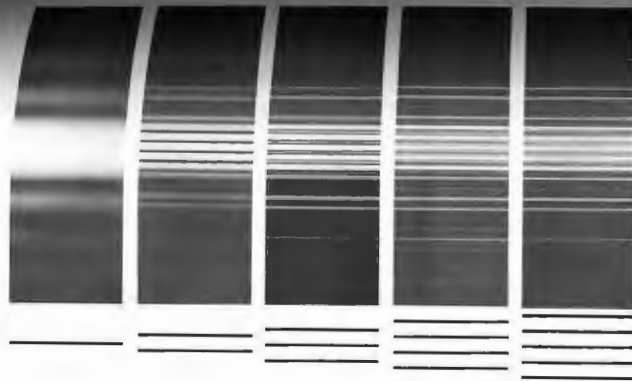
Figure 10.16 Diffraction patterns for slit systems shown at left. (From Weston Sears, Optics. Reprinted with permission of Addison-Wesley Longman.)
