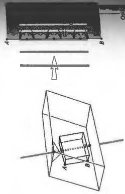
Figure 8.37 A calcite plate cut parallel to the optic axis.
