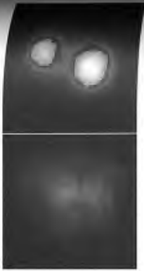
A 1-second exposure of 53 \kappa Ursæ Major using a 1.5-m telescope at Phillips Laboratory. (a) The ordinary uncompensated image is unrecognizable. (b) Using adaptive optics, the image is improved dramatically. (Photos courtesy of Phillips Laboratory, Department of the US Air Force.)
