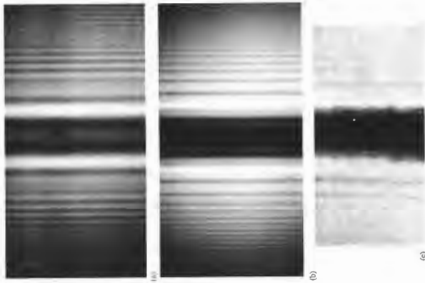
(a) The shadow pattern cast by the lead from a mechanical pencil. (b) The pattern cast by a 1/8-inch diameter rod. (c) Fresnel electron-diffraction pattern of a 2-μm diameter metallized quartz filament. (Photo from O. E. Kemper, Electron Physics , Butterworths, London (1972), pp. 188-191.)
