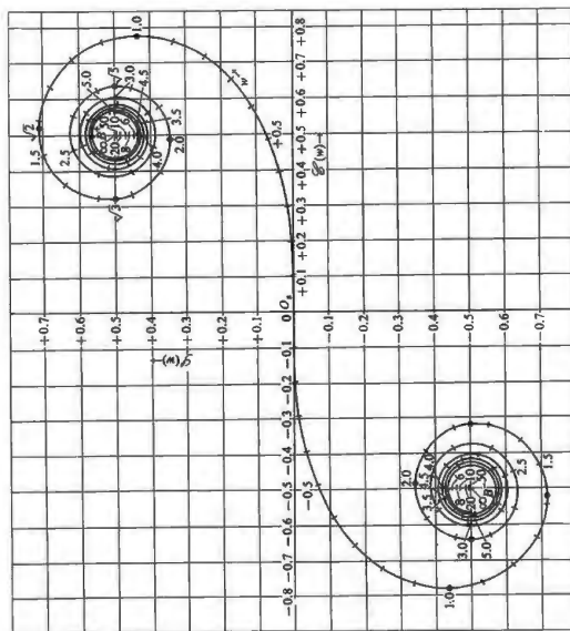
Figure 10.50 The Cornu spiral.
