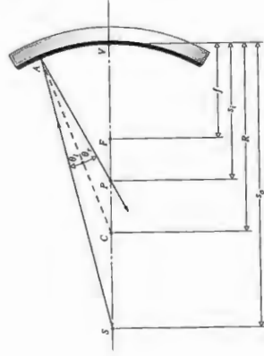
Figure 5.50 A concave spherical mirror. Conjugate foci.
