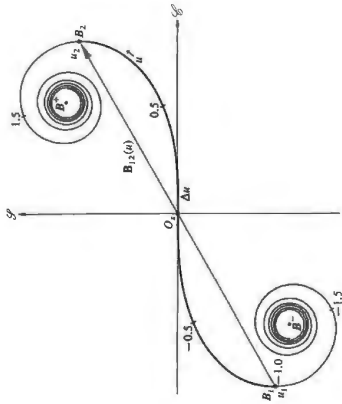
Figure 10.51 Cornu spiral.
