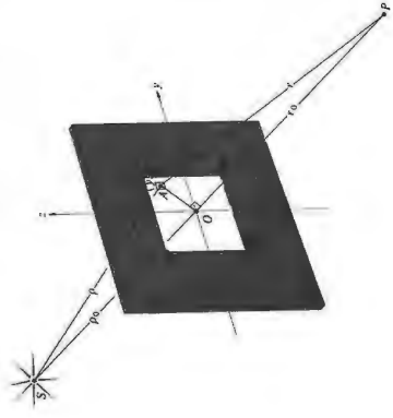
Figure 10.49 Fresnel diffraction at a rectangular aperture.
