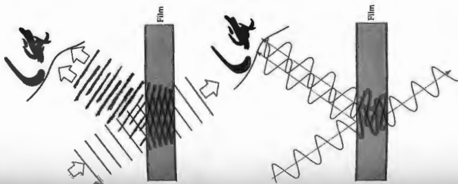
Figure 9.16 The wave and ray representations of thin-film interference. The rays reflected from the top and bottom of the film interfere to create the fringe pattern.
