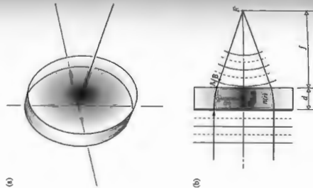
Figure 6.42 (a) A disk of transparent glass whose index of refraction decreases radially out from the central axis. (b) The geometry corresponding to the focusing of parallel rays by a GRIN lens.
