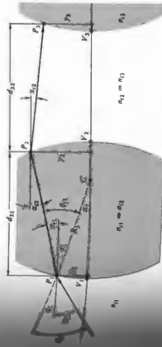
Figure 6.7 Ray geometry.
