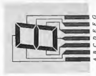
Figure 8.62 A seven-bar electrode array used to display numbers. For example, to form the number 9, a voltage is applied between A and B of the following segments and the large back electrode, D, E, F, and G.
