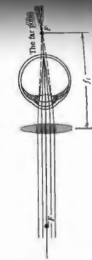
Figure 5.86 Again the far-point distance equals the focal length of the correction lens.
