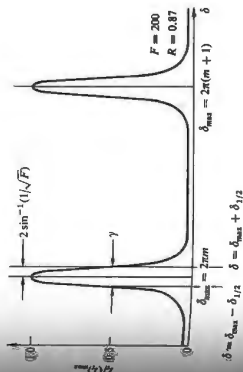
Figure 9.45 Fabry-Perot fringes.
