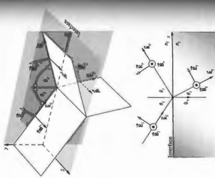
Figure 4.40 An incoming wave whose \vec{E} -field is in the plane-of-incidence.
