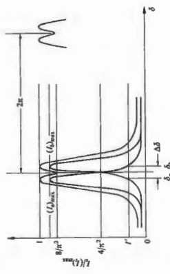
Figure 9.46 Overlapping fringes.
