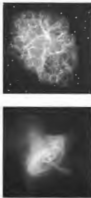
This amazingly detailed X-ray image of the Crab Nebula (see p. 61) was recently taken by the orbiting Chandra X-ray Observatory. The picture reveals the locations of the most energetic particles in the pulsar winds of the pulsar.
