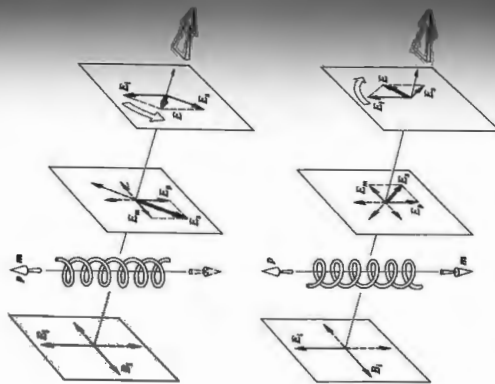
Figure 8.54 The radiation from helical molecules.
