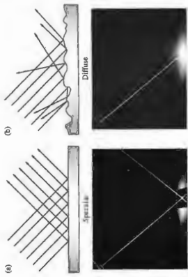
Figure 4.18 (a) Specular reflection. (b) Diffuse reflection. (Photos courtesy Donald Dantz.)
