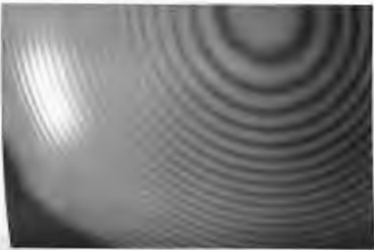
Reference from the thin air film between a convex lens and the flat optical glass it rests on. The illumination was quasimonochromatic. Newton's rings were first studied in depth by Newton and are known as Newton's rings. (Photo by E.H.)
