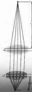
Figure 6.24 A combination of two infinite conjugate lenses yielding a coma-free image at finite conjugates.
