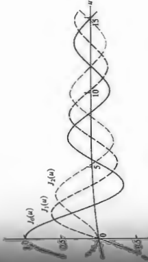
Figure 10.22 Bessel functions.
