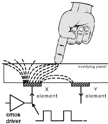
Figure 1-3 Fields With a Conductive Film
