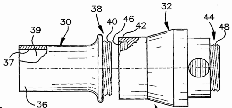
Fig.3 (PRIOR ART)
