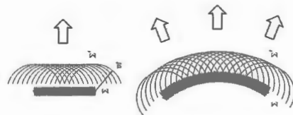
Figure 4.26 According to Huygens's Principle, a wave propagates if the wavefront were composed of an array of point sources, each emitting a spherical wave.
