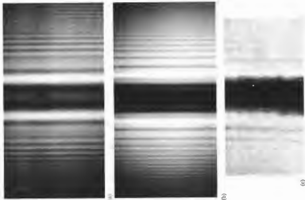
(a) The shadow pattern cast by the lead from a mechanical pencil. (b) The pattern cast by a 1/8-inch diameter rod. (c) Fresnel diffraction pattern of a 2- \mu\text{m} diameter metallized quartz filament. (Photo from O. E. Kemper, Electron Physics , Butterworths, London (1972), pp. 188-191.)
