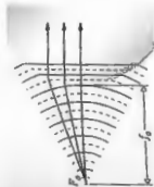
Figure 5.8 Plane waves propagating beyond a spherical interface—spherical waves.
