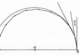
Figure 10.39 Phasor addition.
