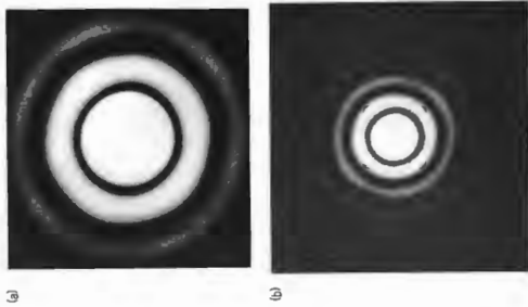
Figure 10.24 Airy rings using (a) a 0.5-mm hole diameter and (b) a 1.0-mm hole diameter. (Photo by E. H.)
