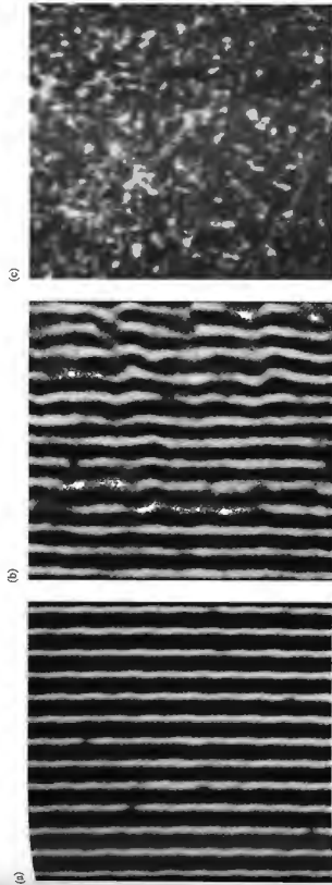
Figure 13.49 Various degrees of modulation of hologram fringes. (Photo courtesy Emmett N. Leith and Scientific American.)
