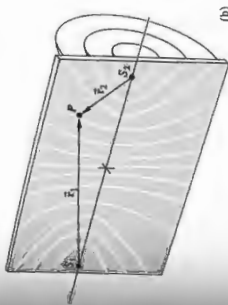
Figure 9.3 (a) Hyperboloidal surfaces of maximum irradiance for two point sources. The quantity m is positive where r_1 > r_2 . (b) Here we see how the irradiance maxima are distributed on a plane containing S_1 and S_2 . (c) The electric-field distribution in the plane shown in part (b). The tall peaks are the point sources S_1 and S_2 . Note that the spacing of the sources is different in (b) and (c). (Photo courtesy, The Optics Project, Mississippi State University.)
