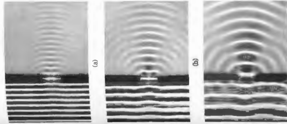
Figure 10.3 Diffraction through an aperture with varying \lambda , as seen in a ripple tank. (a) \lambda > \overline{AB} ; (b) \lambda \approx \overline{AB} ; (c) \lambda < \overline{AB} . (Photo courtesy PSSC Physics, D. C. Heath, Boston, 1960.)
