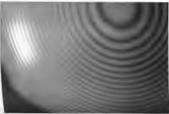
Reference from the thin air film between a convex lens and the flat test glass it rests on. The illumination was quasimonochromatic. Newton's rings were first studied in depth by Newton and are known as Fizeau fringes. (Photo by E.H.)
