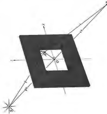
Figure 10.49 Fresnel diffraction at a rectangular aperture.
