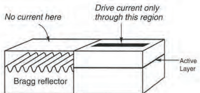
b. Distributed Bragg Reflection Laser.
