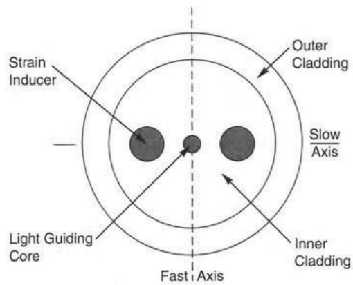
a. PANDA Fiber Cross-Section
