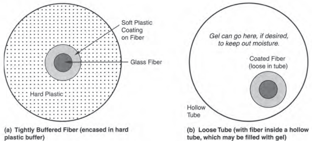
FIGURE 8.5 Tightly buffered and loose-tube structures for cables.
