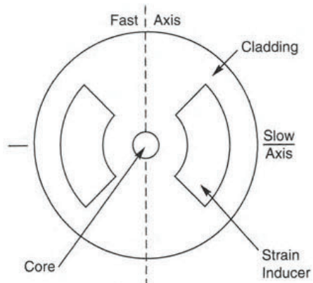
b. Bow-tie Fiber
