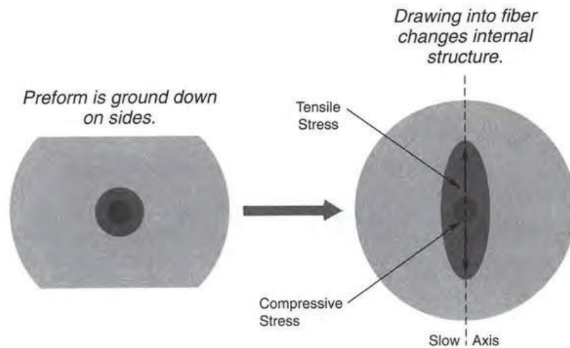
c. Ground Preform Fiber
