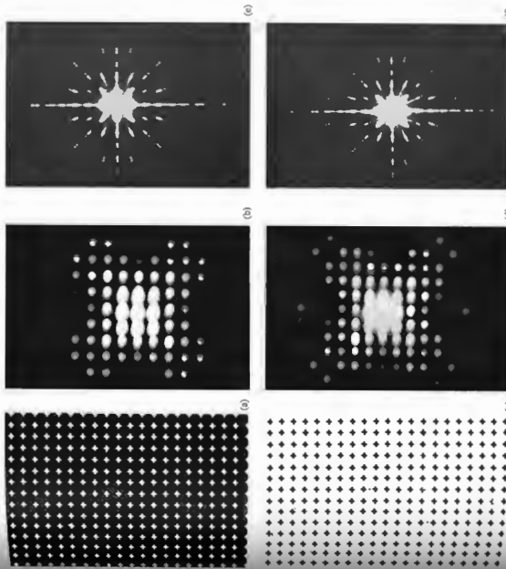
Figure 10.63: (a)-(d) White-light diffraction patterns for regular arrays of apertures and complementary apertures in the form of rounded plus signs. (e) and (f) Diffraction patterns for a regular array of rectangular apertures and complementary apertures in the form of rounded minus signs, respectively. (Photos courtesy the Caling Corporation and Richard B. Hoover.)
