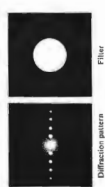
Diffraction pattern
