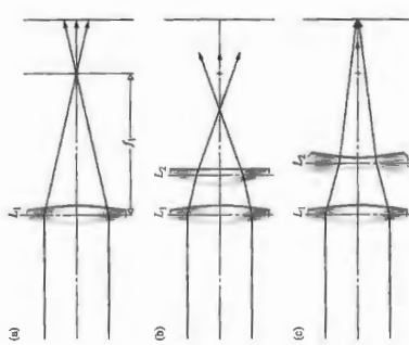
Figure 5.29 (a) The effect of placing a second lens, L_2 , within the focal length of a positive lens, L_1 . (b) When L_2 is positive, its presence adds convergence to the ray bundle. (c) When L_2 is negative, it adds divergence to the ray bundle.
