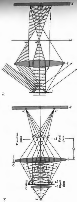
Figure 13.28 Image formation.
