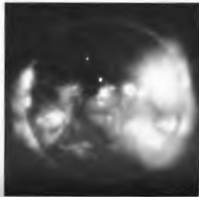
X-ray photograph of the Sun taken March 1970. The limb of the solar disk is visible in the southeast corner. (Photo Courtesy Dr. G. Vaiana and NASA)
