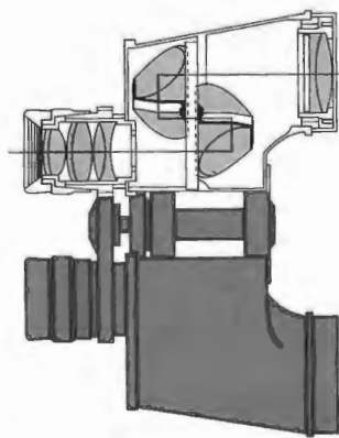
Figure 5.109 A binocular.
