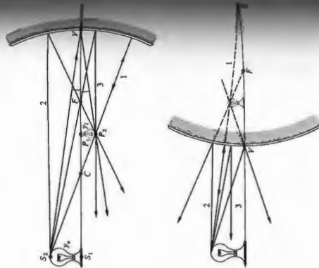
Figure 5.52 Four easy rays to draw. Ray 1 heads toward C and reflects back along itself. Ray 2 comes in parallel to the central axis and reflects toward (or away from) F. Ray 3 passes through (or heads toward) F and reflects off parallel to the axis. Ray 4 strikes point V and reflects such that \theta_i = \theta_r .
