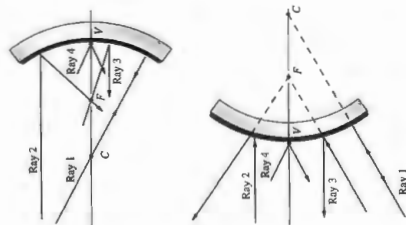
Figure 5.52 Four easy rays to draw. Ray 1 heads toward C and reflects back along itself. Ray 2 comes in parallel to the central axis and reflects toward (or away from) F. Ray 3 passes through (or heads toward) F and reflects off parallel to the axis. Ray 4 strikes point V and reflects such that \theta_i = \theta_r .
