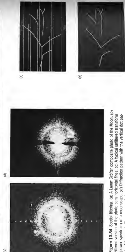
Figure 13.35 Unfiltered and filtered bubble-chamber tracks.
