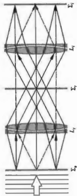
Figure 13.30 Object, transform, and image planes.
