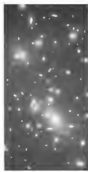
Figure 5.122 Gravitational lensing by a cluster of galaxies. The galaxy cluster Abell 2218 is so massive and compact that light passing through it is deflected by the enormous gravitation field. The process magnifies, brightens, and distorts the images of galaxies that lie far behind it. The numerous arcs in the picture are the contorted images of galaxies 5 to 10 times farther away than the lensing cluster.
