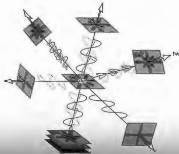
Figure 8.31 Scattering of unpolarized light by a molecule.
