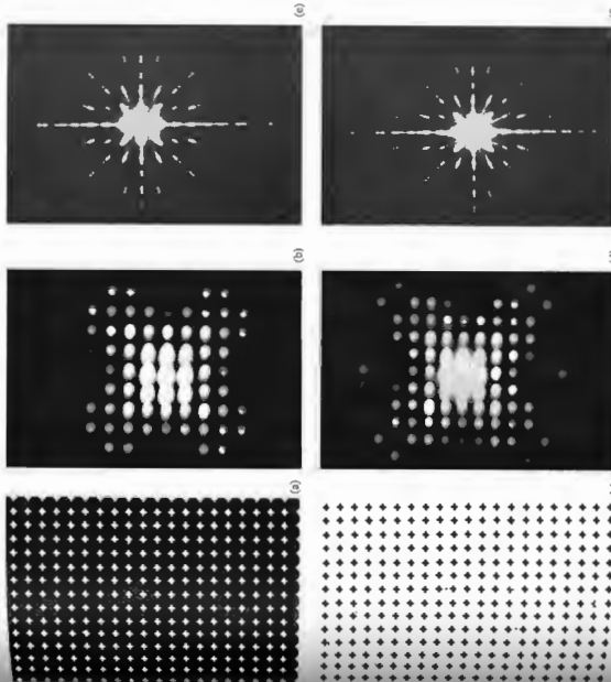
Figure 10.63 White-light diffraction patterns for regular arrays of apertures and complementary obstacles in the form of rounded plus signs. (c) and (d) Diffraction patterns for a regular array of rectangular apertures and obstacles, respectively. (Photos courtesy the Caling Corporation and Richard B. Hoover.)
