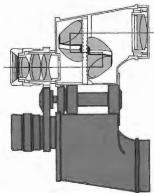
Figure 5.109 A binocular.
