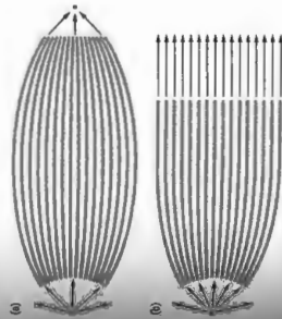
Figure 5.79 A bundle of multicapillary threads used to (a) focus or (b) collimate X-rays from a point source.
