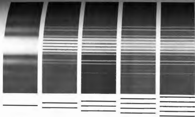
Figure 10.16 Diffraction patterns for slit systems shown at left. (mgz) Weston Sears, Optics. Reprinted with permission of Addison-Wesley Longman.
