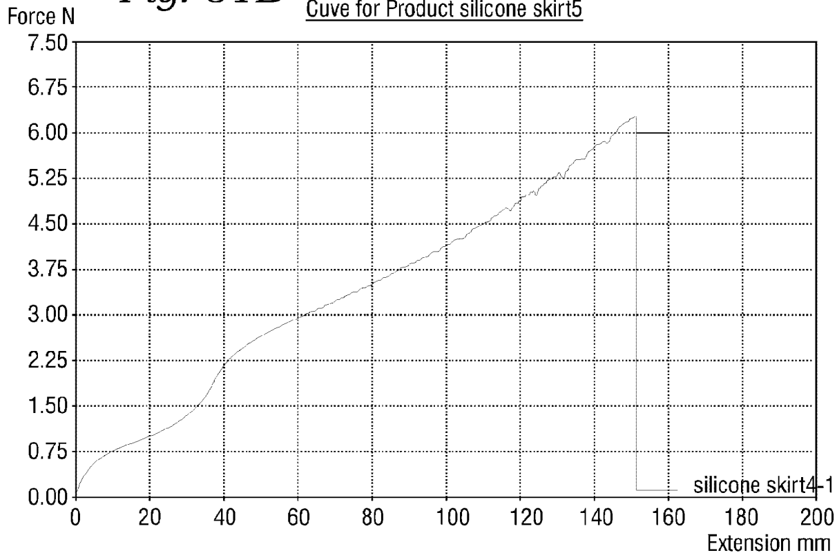
Fig. 31C Curve for Product silicone skirt4
