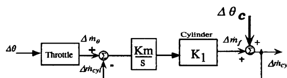
Figure 4: Block diagram of the linearized breathing process.
