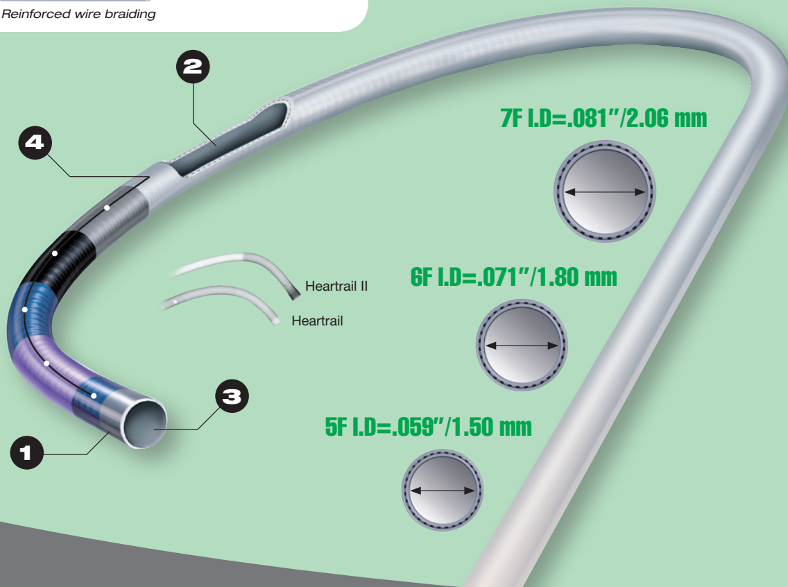
Reinforced wire braiding
