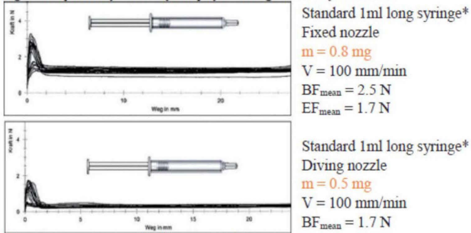
Fig. 5: Extrusion force profile after optimized siliconization.
