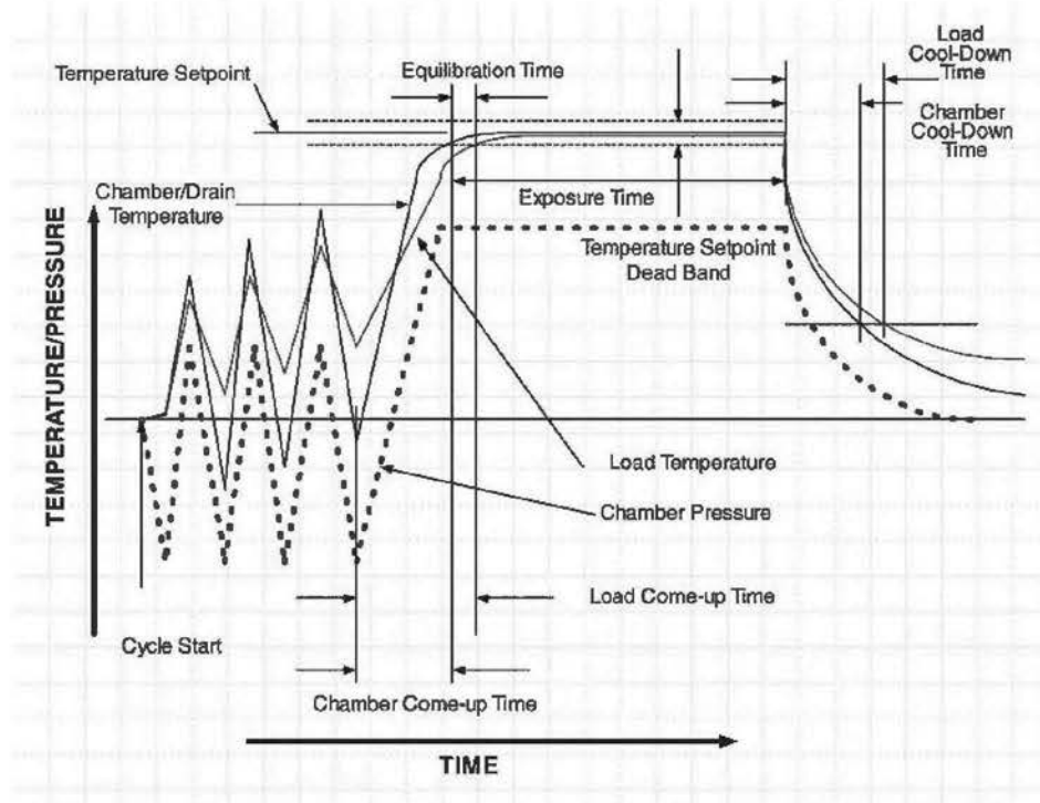
Figure 9 Multiple prevacuum cycle.
