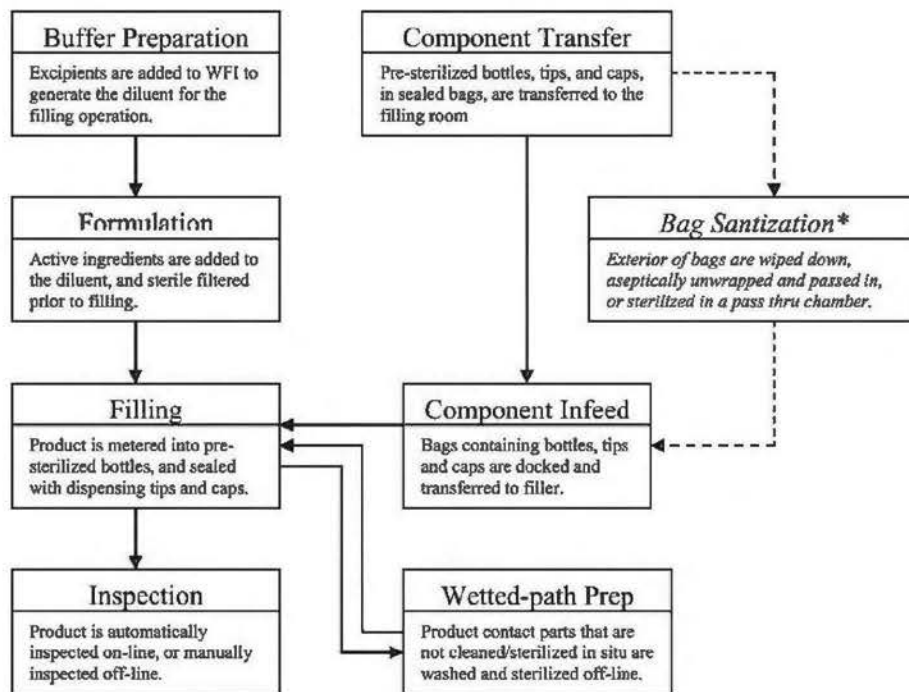
Figure 21 Process flow, plastic bottle. *Not required if isolation fill technology is used.
