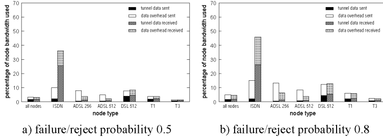
Figure 8.14: Bandwidth usage with failed and rejected tunnels.
