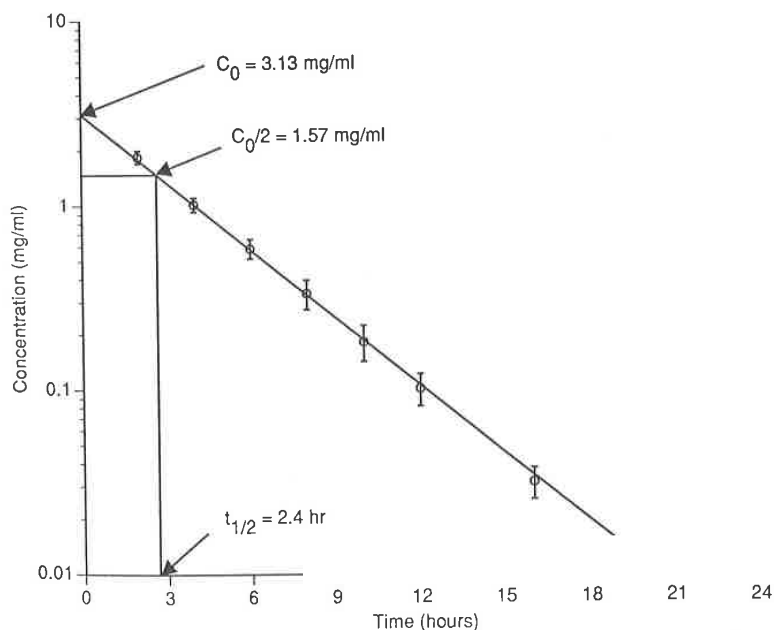
Fig. 3 Semilogarithmic plot of concentration versus time for the hydrolysis of ethyl acetate. (Data shown in Table 2; one standard deviation is in error bars.)
