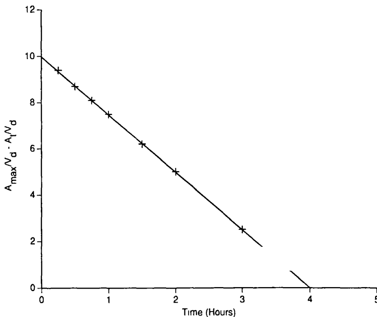
Fig. 12 Plot of the residuals (crosses)
