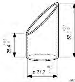
Figure 3 – Ingestion gauge
