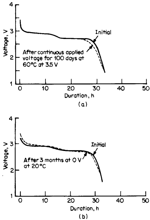
FIGURE 34.42 Overcharge and overdischarge characteristics of \text{LiAl}/\text{V}_2\text{O}_5 coin-type battery (VL2020 size): (a) overcharge characteristics, (b) overdischarge characteristics (charge at 200\ \Omega for 48 h, discharge at 3\ \text{k}\Omega ). (From Panasonic Division of Matsushita Electric Corp. of America.)
