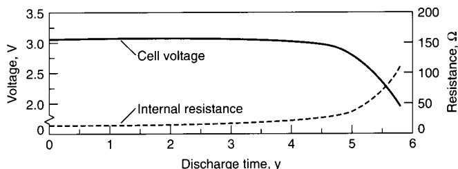
FIGURE 14.57 Internal resistance of Li/MnO 2 coin-type battery (280-mAh size), 5- \mu A drain, at 20°C.
