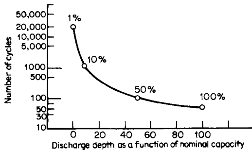
FIGURE 34.43 Cycle life vs. depth of discharge (%) for a \text{LiAl}/\text{V}_2\text{O}_5 coin-type battery (VL2020 size) at 20^\circ\text{C} . (From Panasonic Division of Matsushita Electric Corp. of America.)
