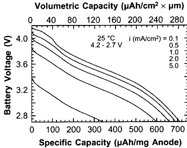
FIGURE 35.108 Rate capability of a SiTON/LiPON/LiCo 2 battery. Specific capacity and volumetric capacity are based on the as-deposited mass and volume of SiTON. (Courtesy of Oak Ridge National Laboratory. Reproduced from the Journal of Power Sources , Vol. 81, 1999, with permission from Elsevier Science.)
