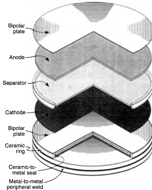
FIGURE 41.2 Exploded view of four-cell bipolar Li-Al/FeS x stack under development for electric-vehicle applications shown electrodes, separator, and bipolar plate current collector. (Courtesy of Argonne National Laboratory.)
