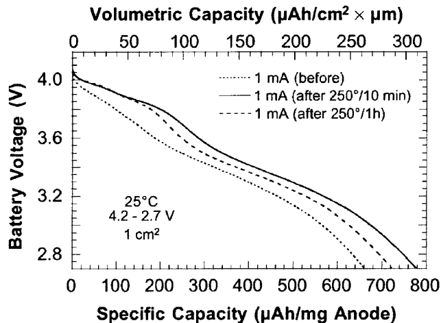
FIGURE 35.109 Voltage of a SiTON/LiCo 2 battery when discharged at 25°C at 1 mA/cm 2 before and after heat treatment at 250°C for 10 minutes or 1 hour. (Courtesy of Oak Ridge National Laboratory. Reproduced from the Journal of Power Sources , Vol. 81, 1999, with permission from Elsevier Science.)
