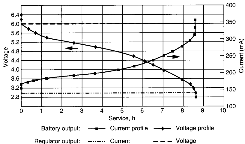
FIGURE 3.18 Characteristics of a voltage regulator. Battery output—1 W; regulator output—840 mW.
