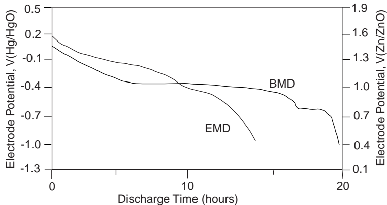
FIGURE 36.2 Discharge curve for electrolytic Manganese Dioxide (EMD) and Bismuth modified Manganese Dioxide (BMD) in KOH. (Courtesy of Rechargeable Battery Corp.)
