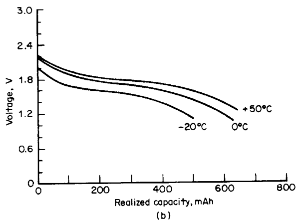
FIGURE 34.14 Discharge characteristics of Li/MoS 2 battery. Battery charged at 20°C, 60 mA to 2.4 V. (a) Discharge characteristics at 20°C. (b) Discharge characteristics at 120 mA. (From Moli Energy Ltd.)
