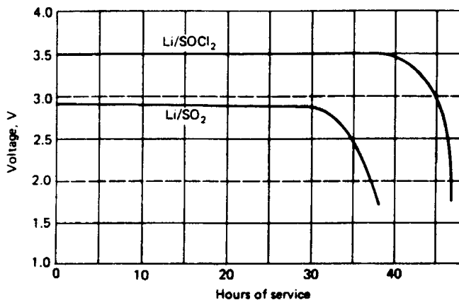
FIGURE 14.2 Comparison of performance of \text{Li}/\text{SO}_2 and \text{Li}/\text{SOCl}_2 C-size batteries; 100-mA discharge load at 20^\circ\text{C} .
