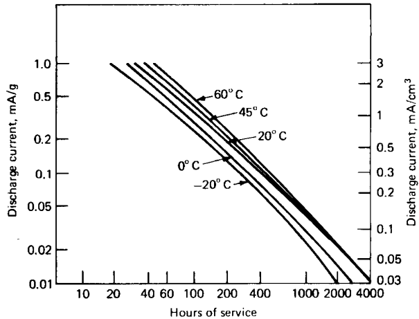
FIGURE 14.67 Service life of Li/(CF) n coin-type batteries at various discharge rates and temperatures; 2.0-V end voltage.
