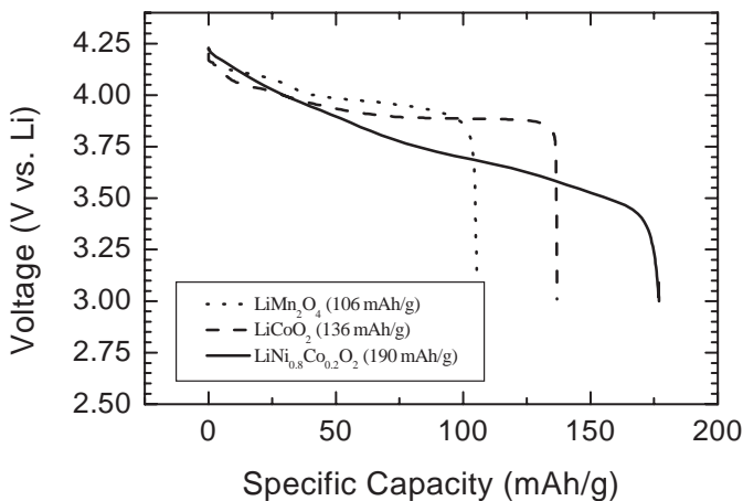
FIGURE 35.9 Voltage and specific capacity of common positive electrode materials on the first discharge at the C/20 rate. The LiNi 1-x Co x O 2 materials were discharged at 0.16 mA/cm 2 , the LiCoO 2 at 7.5 mA/g, and the LiMn 2 O 4 at 0.09 mA/cm 2 . (Courtesy of FMC and Yardney Technical Products, Inc.)
