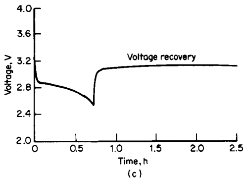
FIGURE 34.32 (a) Discharge/charge behavior of a Li/LiAlCl 4 · 6SO 2 C-size battery at 1 mA/cm 2 . Voltage limits; 2.8–4.0 V. Line—battery, symbols (Δ)—cathode vs. ref. (b) High-rate pulse discharge of a Li/LiAlCl 4 · 6SO 2 C-size battery. Pulse rate at 20 mA/cm 2 for 20 s. Rest period for 180 s. (c) Discharge characteristics and voltage recovery (without load) of a Li/LiAlCl 4 · 6SO 2 C-size battery at -20°C. Discharge at 3.2 mA/cm 2 . (From Yardney Technical Products, Inc.)
