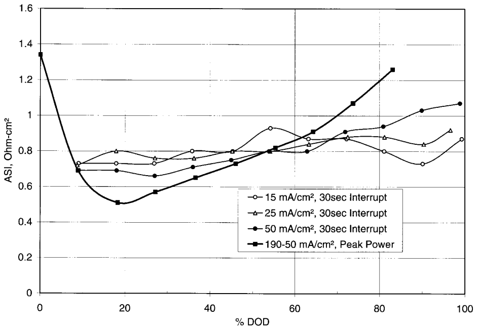
FIGURE 41.10 ASI vs. DOD for a 3-cm diameter cell with 12-mol % CoS 2 additive to the Fe 2 S 2 positive electrode. ASI determined from 30-second current interrupts at various discharge current rates and also from USABC peak power test. (From Henriksen, et al. 8 )
