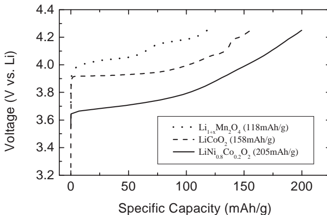
FIGURE 35.8 Voltage and specific capacity of common positive electrode materials on the first charge at 25°C. All materials were charged at approximately C/20, the LiCoO 2 at 7.2 mA/g, the LiNi 1-x Co x O 2 materials at 0.16 mA/cm 2 , and the LiMn 2 O 4 at 0.09 mA/cm 2 . (Courtesy of FMC and Yardney Technical Products, Inc.)
