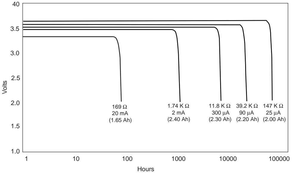
FIGURE 14.20 Discharge characteristics of high-capacity Li/SOCl 2 cylindrical AA-size bobbin battery on low-rate discharge at +25°C. (Ref. 23.)
