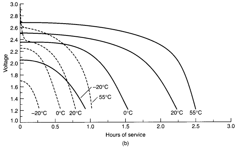
FIGURE 14.51 Discharge characteristics of cylindrical (spirally wound electrode) Li/MnO 2 battery (CR123A-size). (a) Discharge at 30 and 125 mA. Broken line—125 mA; solid line—30 mA. (b) Discharge at 500 and 1000 mA. Broken line—1 A; solid line—0.5 A. (b) Discharge at 500 and 1000 mA. Broken line—1 A; solid line—0.5 A.
