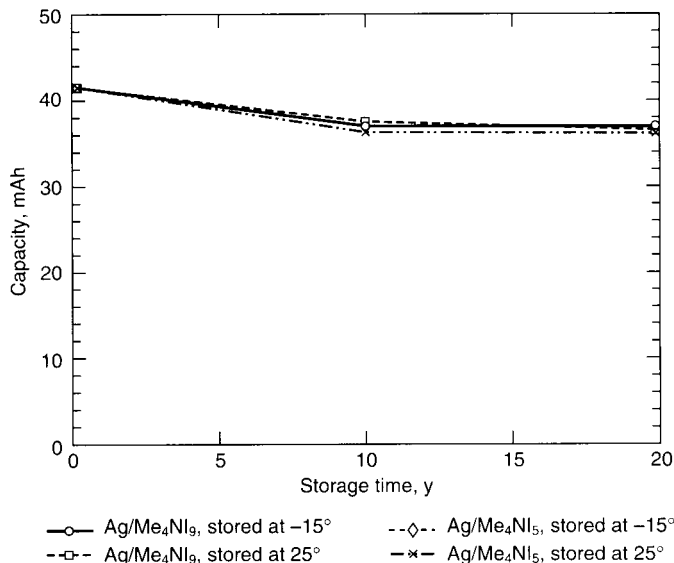
FIGURE 15.25 Capacity of \text{Ag}/\text{RbAg}_4\text{I}_5/\text{Me}_4\text{NI}_n batteries as a function of storage time. (From Ref. 29.)
