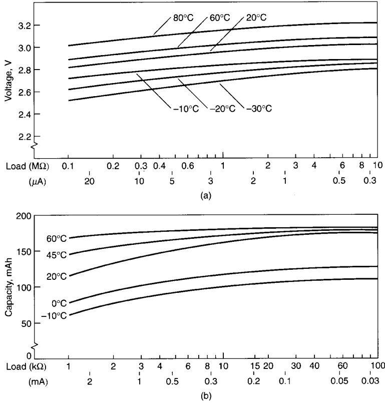
FIGURE 14.66 Discharge characteristics of Li/(CF) n coin-type battery (165-mAh size). (a) Operating voltage vs. discharge load; voltage at 50% discharge. (b) Capacity vs. discharge load; cutoff at 2.0 V. (Courtesy of Panasonic, Division of Matsushita Electric Corp. of America.)
