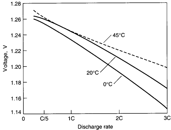
FIGURE 28.11 Midpoint discharge voltage vs. rate at various temperatures for sealed nickel-cadmium batteries, 1-V cutoff.
