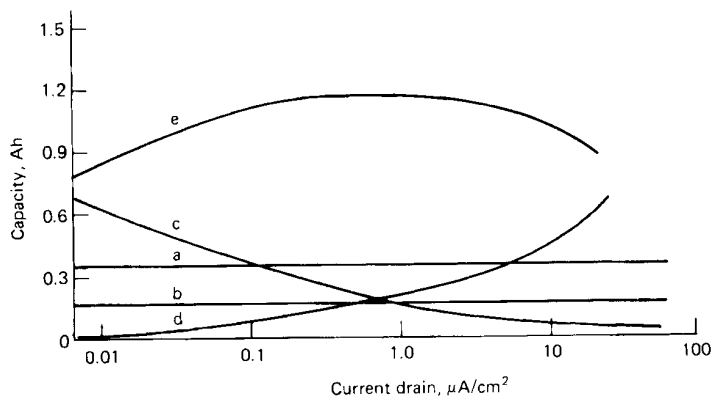
FIGURE 15.19 Capacity and loss projections for 2.0-Ah stoichiometric capacity Li/I 2 battery. a —loss to 1:1 adduct formation; b —loss to iodination reaction; c —projected loss to self-discharge; d —projected loss to polarization; e —net utilizable battery capacity. (Courtesy of Medtronic, Inc.)
