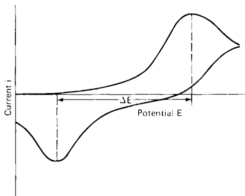
FIGURE 2.22 Cyclic voltammogram of a quasi-reversible process.
