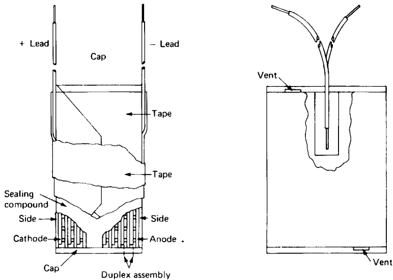
FIGURE 17.1 Seawater battery, immersion type.
