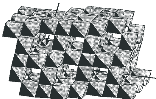
\lambda\text{-MnO}_2
