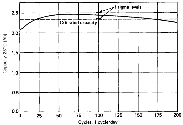
FIGURE 24.19 Effect of cycling on cell capacity, VRLA cell, C/5 discharge rate. Rated at 2.35 Ah at C/5 rate.
