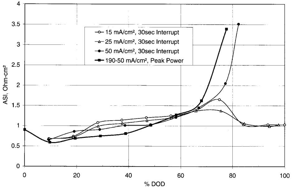
FIGURE 41.9 ASI vs. DOD for a 3-cm diameter cell with Fe 2 S 2 positive electrode. ASI determined from 30-second current interrupts at various discharge current rates and also from USABC peak power test. (From Henriksen, et al. 8 )
