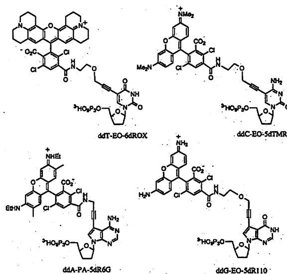
Figure 1. Structure of the d-rhodamine dye-labeled terminators.
