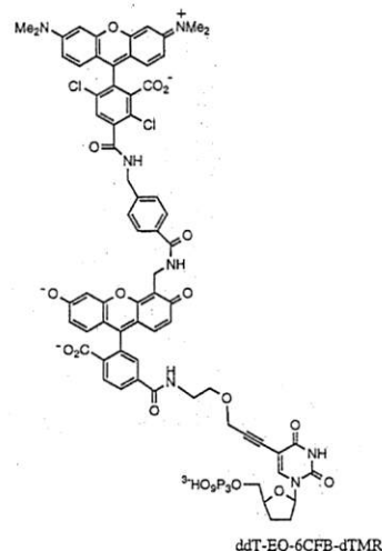
Figure 2. Structure of the ddT-BigDye terminator.
