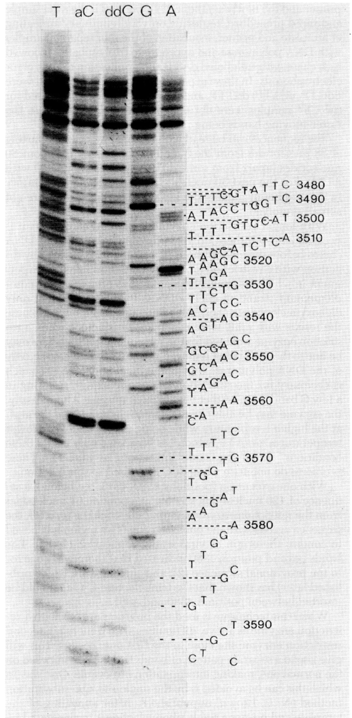
FIG. 3. Autoradiograph of an experiment with fragment A8 as primer on the viral strand of \phi X174 DNA using the single-site ribo-substitution method. Electrophoresis was on a 12% gel at 40 mA for 6 hr. The top 5.5 cm is not shown. Inhibitors used were (left to right) ddTTP, araCTP, ddCTP, ddGTP, and ddATP.
