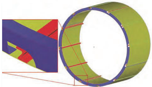
FIGURE 2: Typical fabricated structure with solid geometry.
