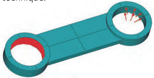
FIGURE 1: Component loaded and constrained at surface geometry.
