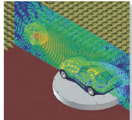
Simulating the electric field distribution and antenna radiation far field pattern at 1 GHz for a complete vehicle simulation, according to ISO 11451-2, using the conventional finite element method approach. The simulation was done using ANSYS software.
