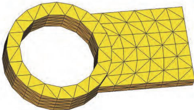
FIGURE 6: Global mesh control.
