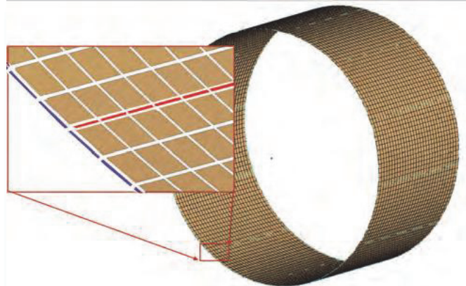
FIGURE 3: Typical fabricated structure and mesh.
