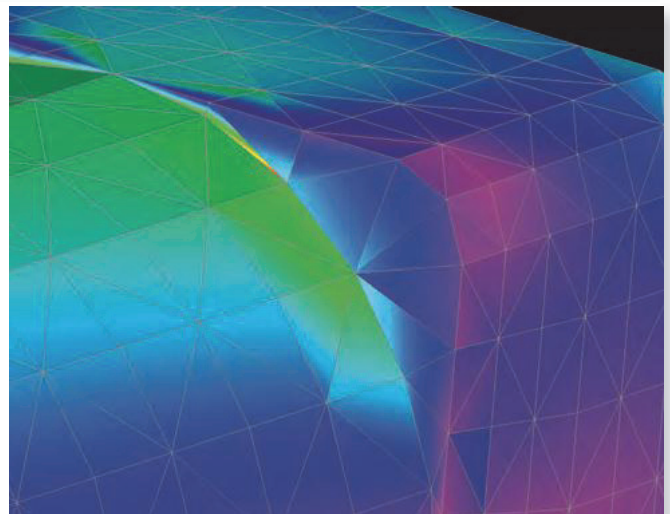
← FIGURE 7: Curvature-based mesh refinement.
