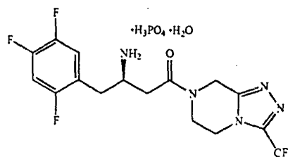
(2R)-4-oxo-4-[3-(trifluoromethyl)-5,6-dihydro[1,2,4]triazolo[4,3-a]pyrazin-7(8H)-yl]-1-(2,4,5-trifluorophenyl)butan-2-amine dihydrogenphosphate monohydrate
