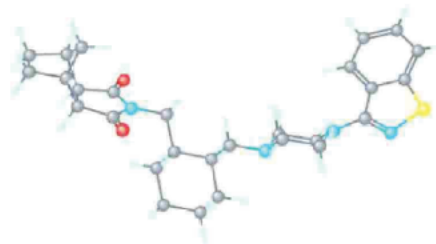
Figure 1 Three-dimensional structure of lurasidone, also known as (3 a R,4 S ,7 R ,7 a S)-2-[(1 R ,2 R )-2-[4-(1,2-benzisothiazol-3-yl)piperazin-1-ylmethyl]cyclohexylmethyl]hexahydro-4,7-methano-2 H -isoindole-1,3-dione hydrochloride or Latuda.
