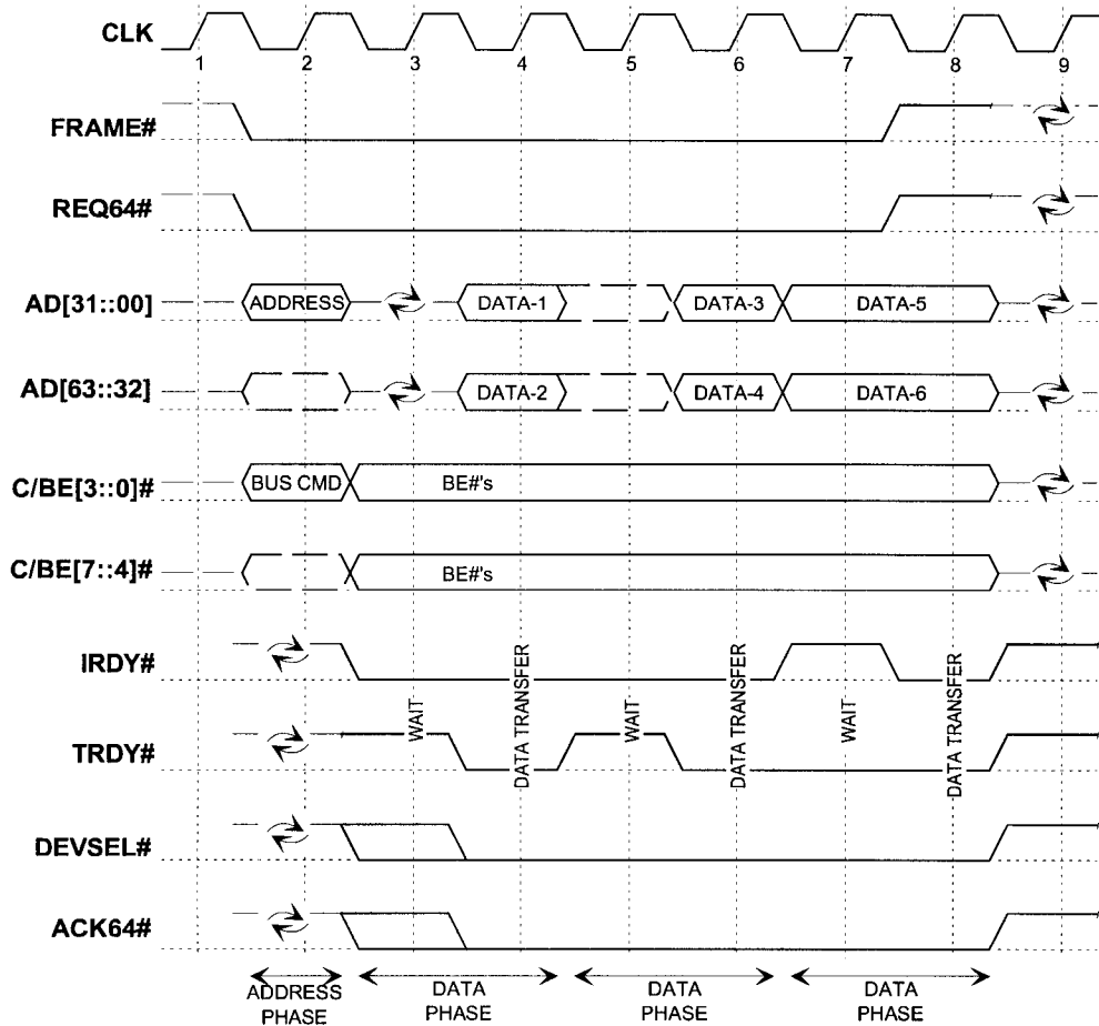
Figure 3-31: 64-bit Read Request with 64-bit Transfer
