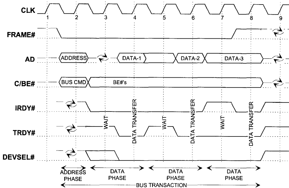
Figure 3-1: Basic Read Operation
