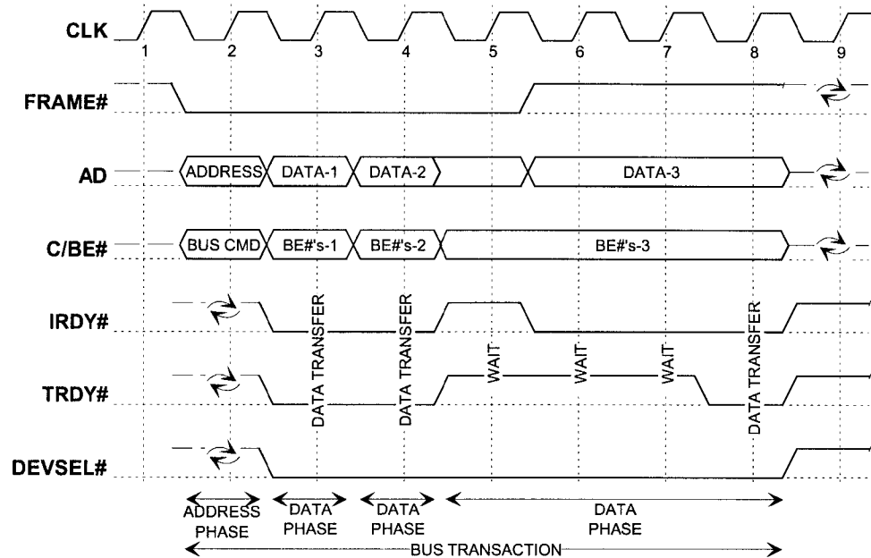
Figure 3-2: Basic Write Operation
