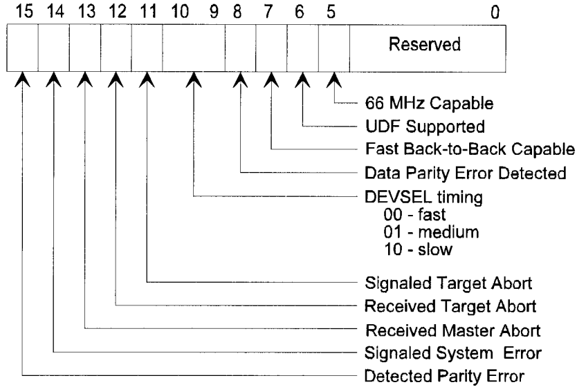
Figure 6-3: Status Register Layout
