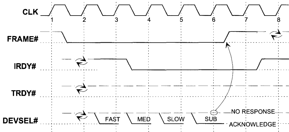
Figure 3-4: Master-Abort Termination
