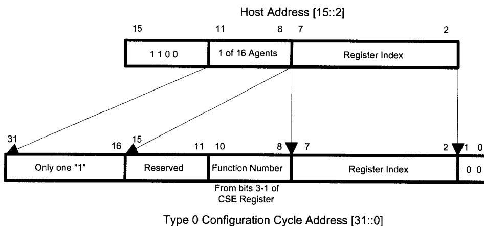
Figure 3-23: Translation to Type 0 Configuration Cycle
