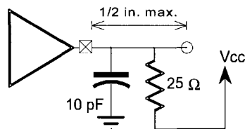
Figure 7-7: T_{val(max)} Falling Edge
