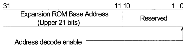
Figure 6-7: Expansion ROM Base Address Register Layout
