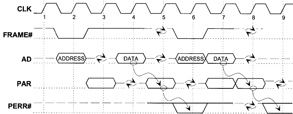
Figure 3-26: Parity Operation
