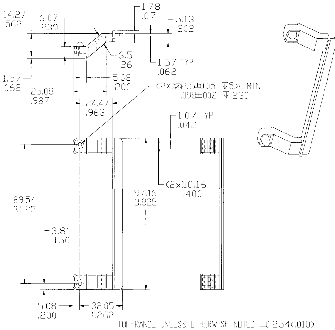
Figure 5-13: ISA Retainer
