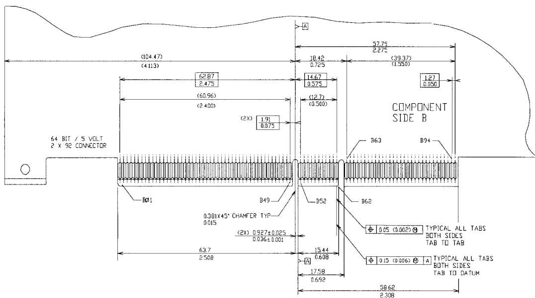
Figure 5-25: 5V/64-bit Card Edge Connector Dimensions and Tolerances
