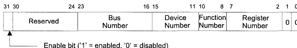
Figure 3-20: Layout of CONFIG_ADDRESS Register
