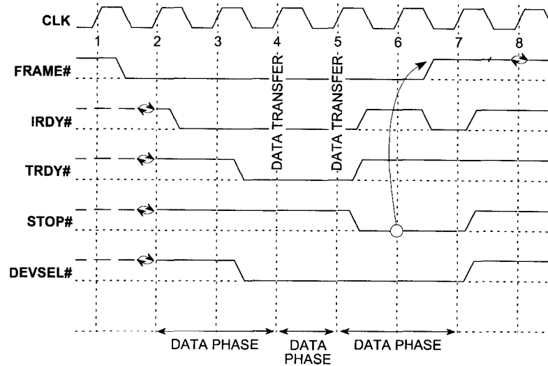
Figure 3-9: Disconnect-2 Without Data Termination
