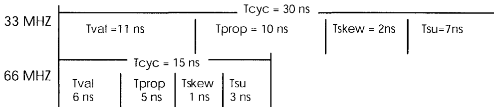
Figure 7-2: 33 MHz PCI vs. 66 MHz PCI Timing
