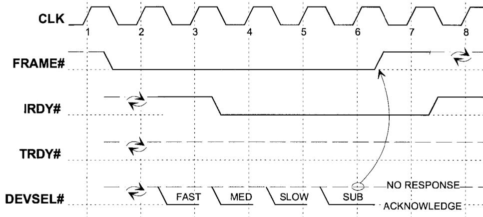
Figure 3-16: DEVSEL# Assertion
