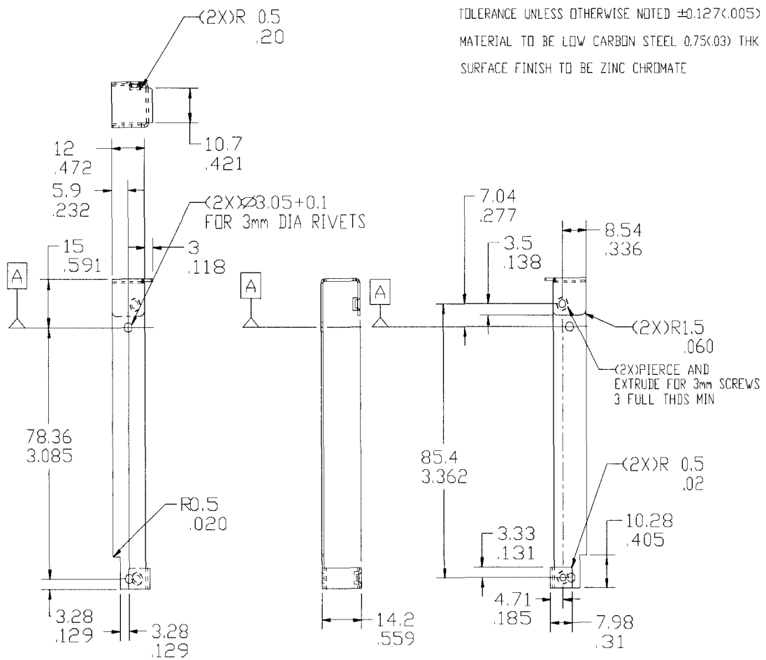
Figure 5-14: MC Bracket Brace
