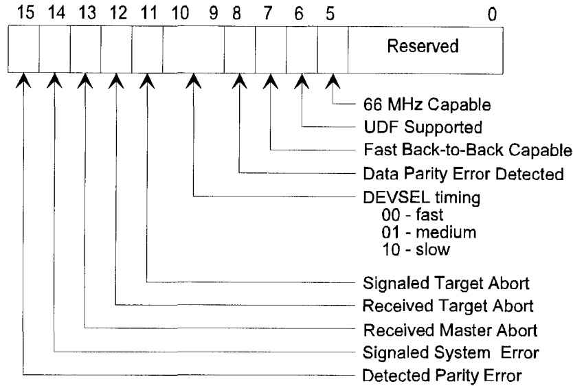
Figure 7-1: Status Register Layout
