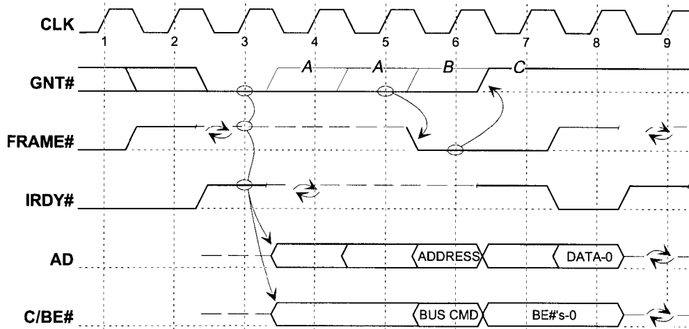
Figure 3-17: Address Stepping
