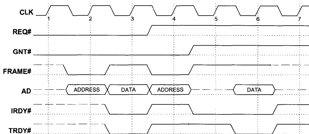
Figure 3-12: Arbitration for Back-to-Back Access
