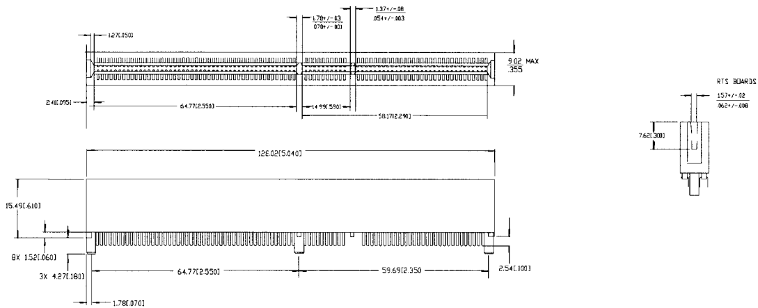
Figure 5-20: 5V/64-bit Connector
