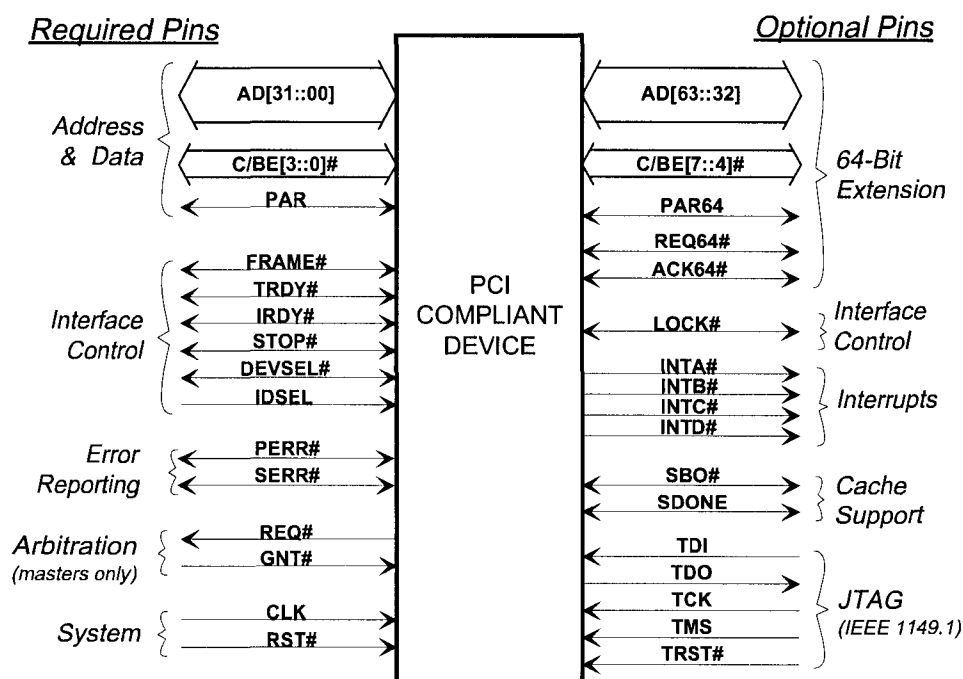
Figure 2-1: PCI Pin List
