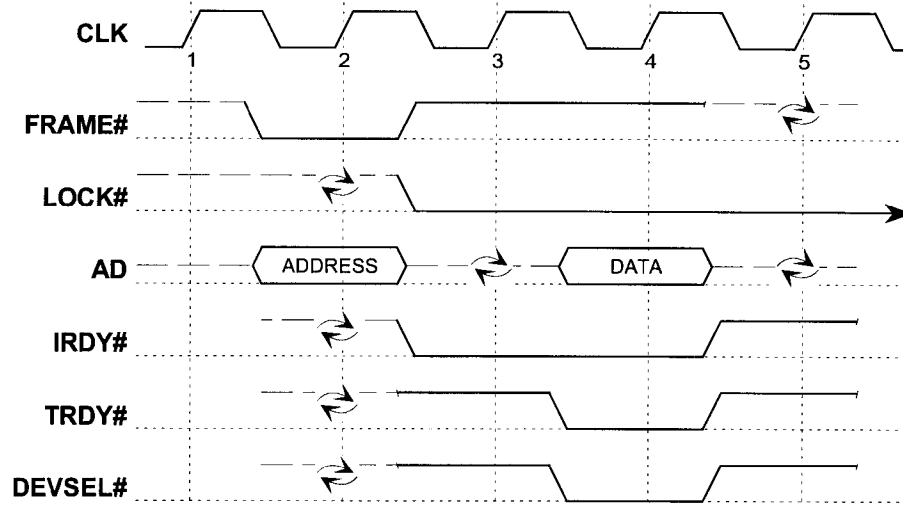
Figure 3-13: Starting an Exclusive Access
