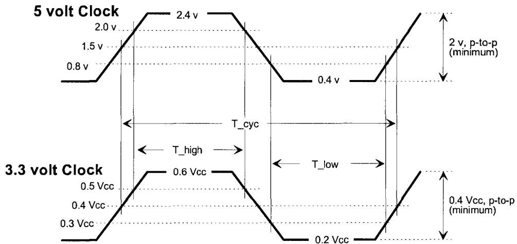
Figure 4-7: Clock Waveforms
