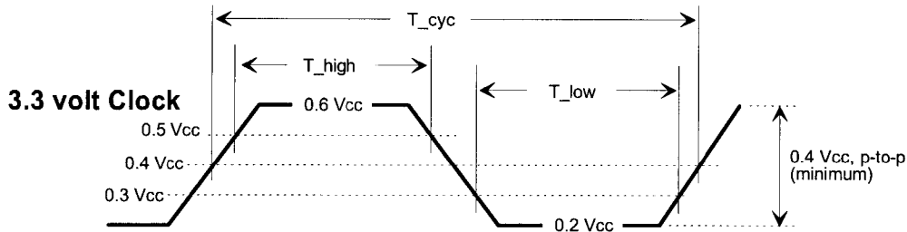
Figure 7-3: 3.3V Clock Waveform
