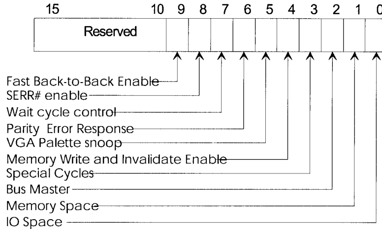
Figure 6-2: Command Register Layout
