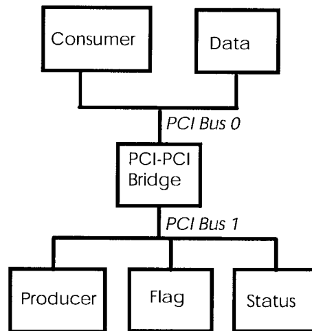
Figure E-1: Example Producer - Consumer Model
