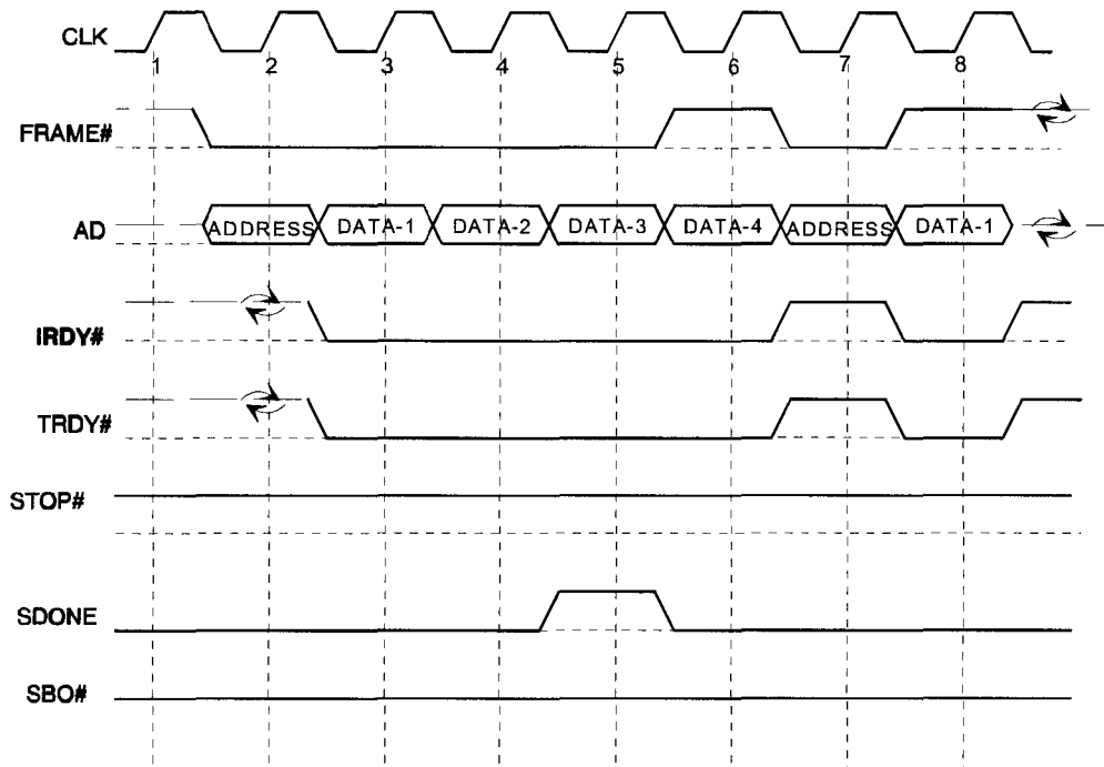
Figure 3-29: Memory Write and Invalidate Command
