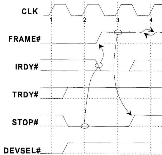
Figure 3-10: Target-Abort
