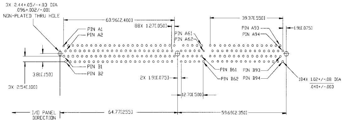
Figure 5-21: 5V/64-bit Connector Layout Recommendation
