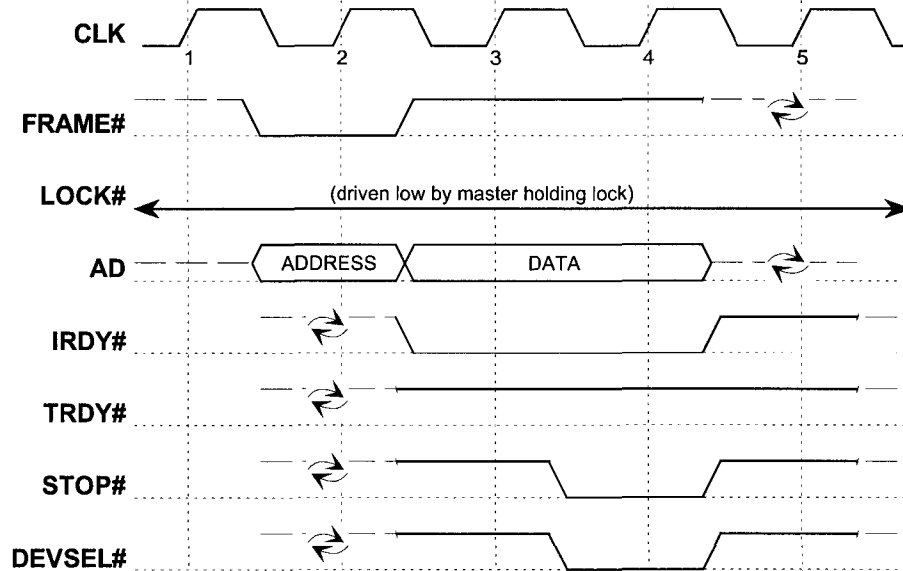
Figure 3-15: Accessing a Locked Agent
