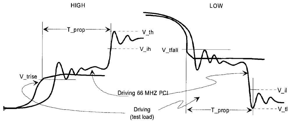
Figure 7-11: Measurement of T_{prop}
