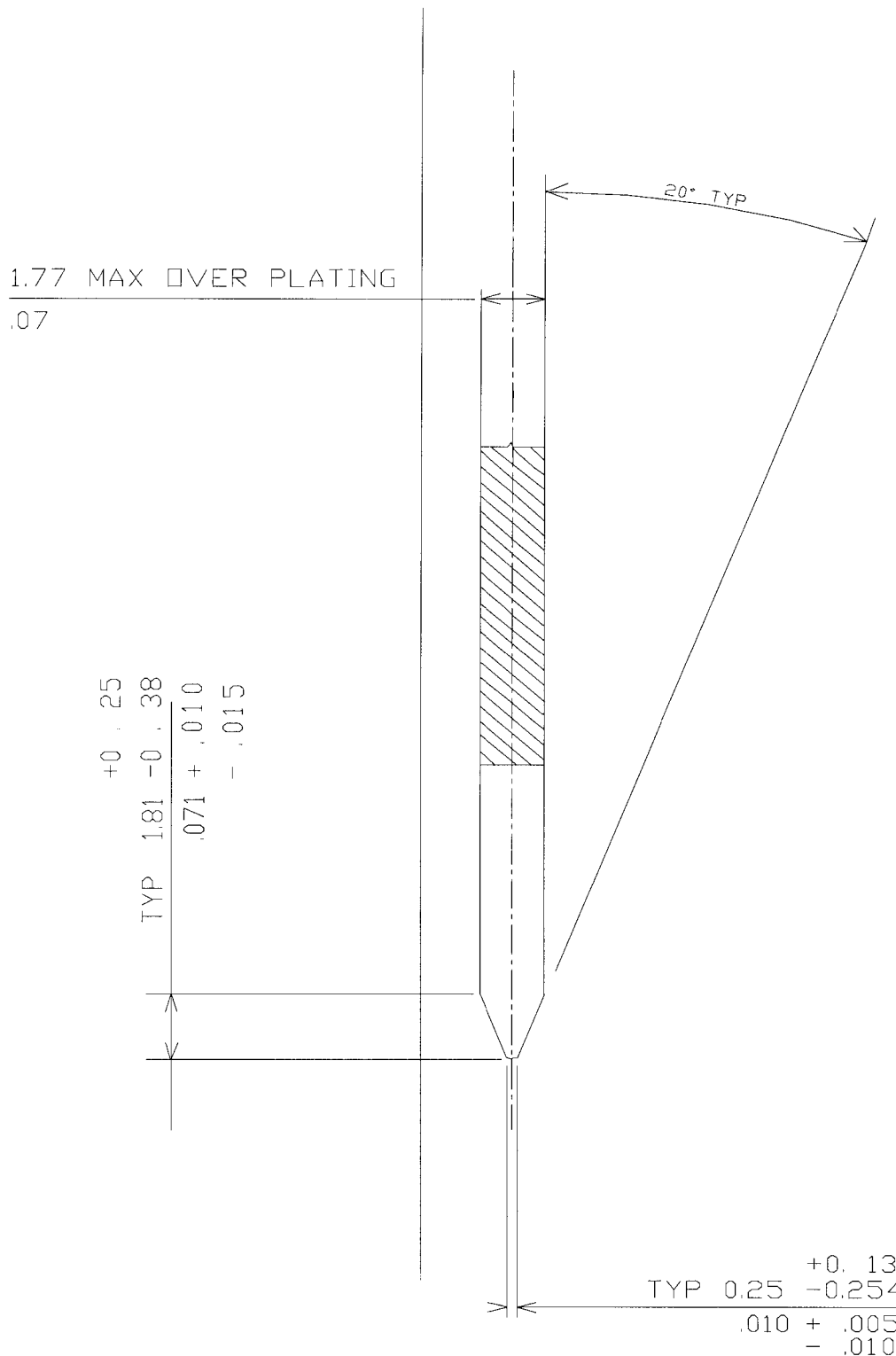
Figure 5-7: PCI Card Edge Connector Bevel
