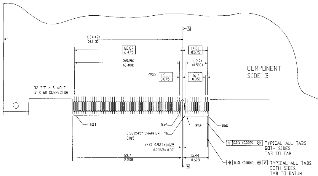
Figure 5-24: 5V/32-bit Card Edge Connector Dimensions and Tolerances
