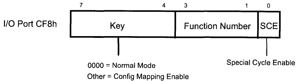
Figure 3-22: Configuration Space Enable Register Layout
