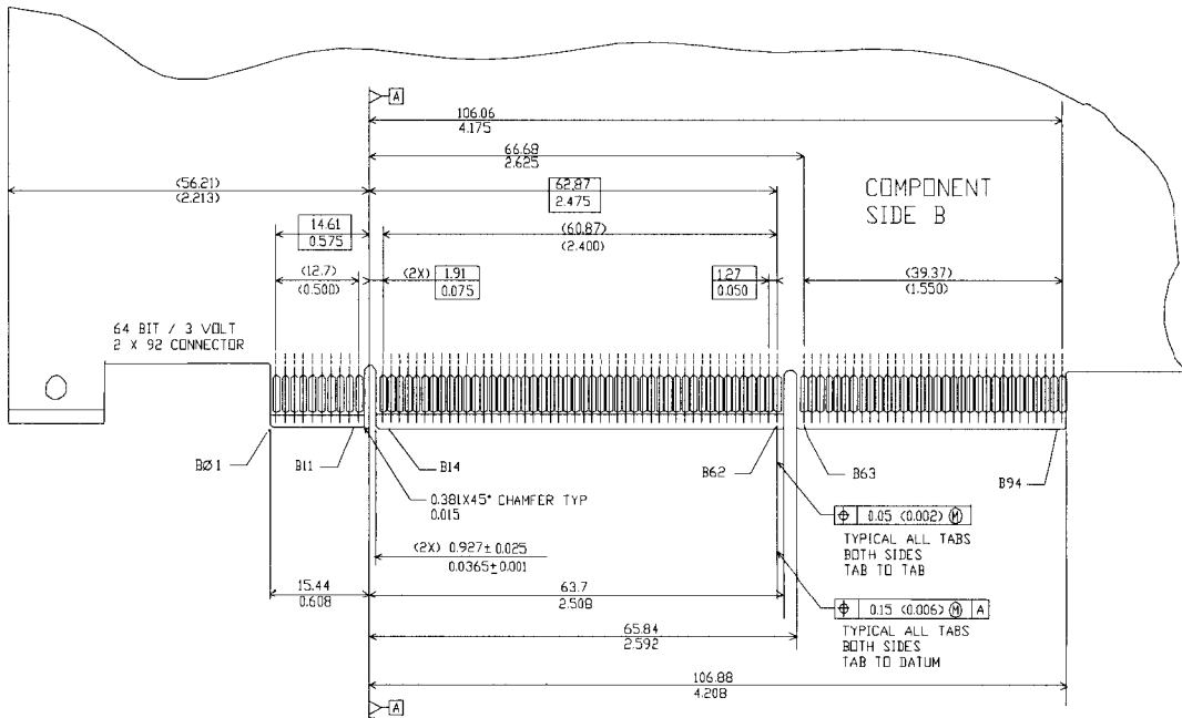
Figure 5-27: 3.3V/64-bit Card Edge Connector Dimensions and Tolerances
