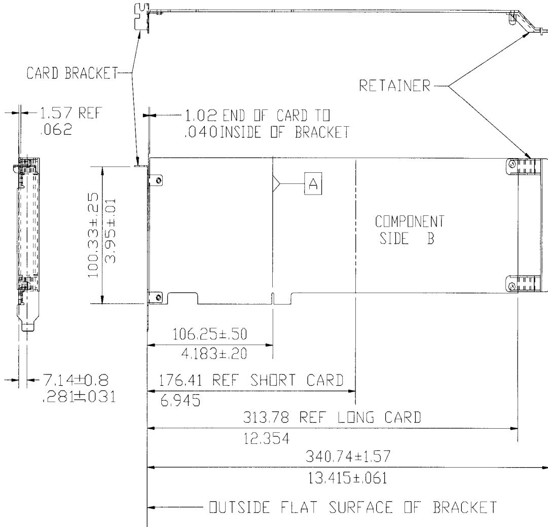
Figure 5-8: ISA Assembly (5V)
