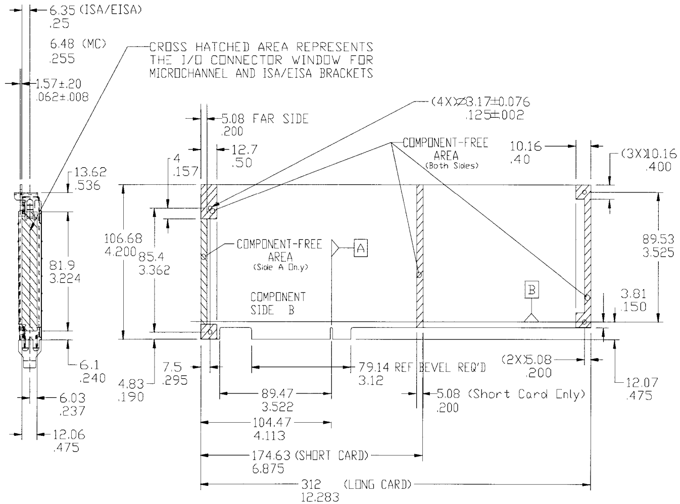
Figure 5-1: PCI Raw Card (5V)
