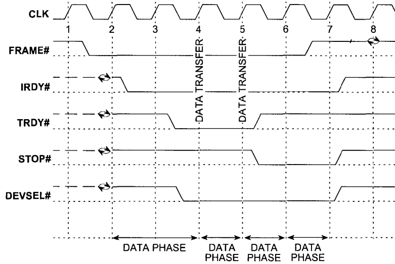
Figure 3-8: Disconnect-1 Without Data Termination
