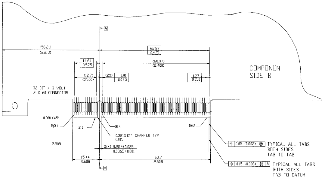
Figure 5-26: 3.3V/32-bit Card Edge Connector Dimensions and Tolerances
