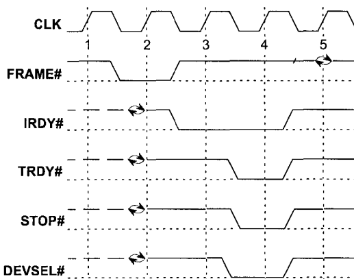
Figure 3-7: Master Completion Termination
