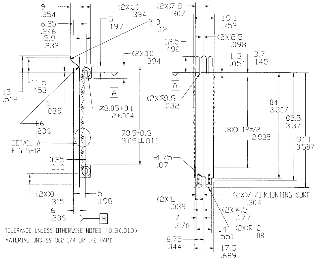
Figure 5-15: MC Bracket
