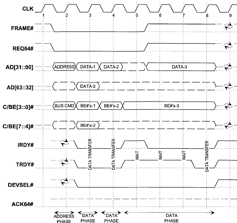
Figure 3-32: 64-bit Write Request with 32-bit Transfer
