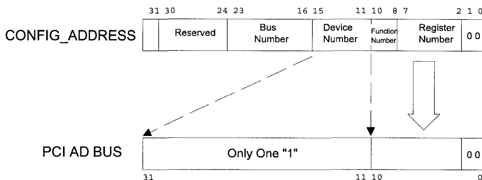
Figure 3-21: Bridge Translation for Type 0 Configuration Cycles
