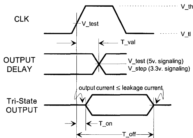
Figure 4-8: Output Timing Measurement Conditions
