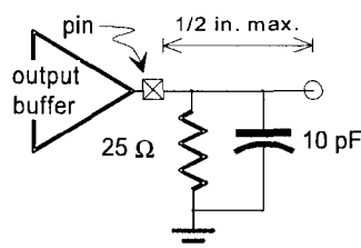
Figure 7-6: T_{val(max)} Rising Edge
