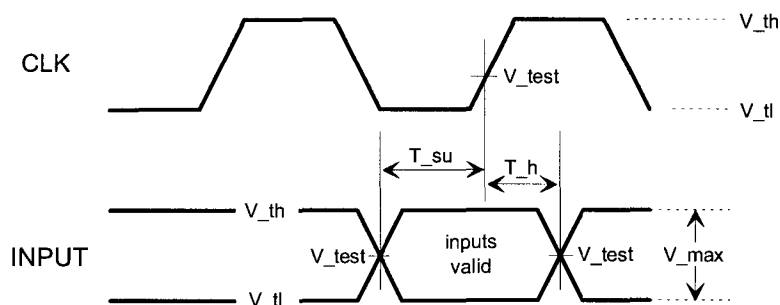
Figure 4-9: Input Timing Measurement Conditions
