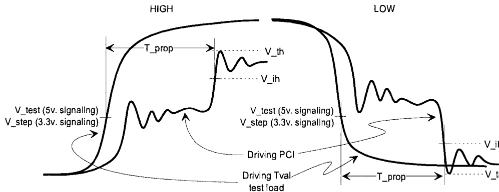
Figure 4-13: Measurement of T_{prop}
