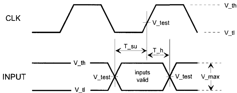
Figure 7-5: Input Timing Measurement Conditions
