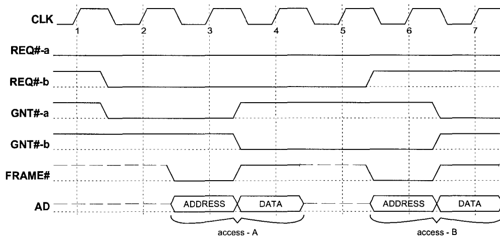
Figure 3-11: Basic Arbitration
