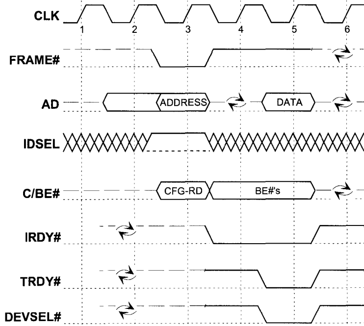
Figure 3-18: Configuration Read
