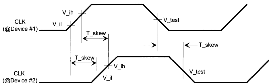
Figure 4-11: Clock Skew Diagram
