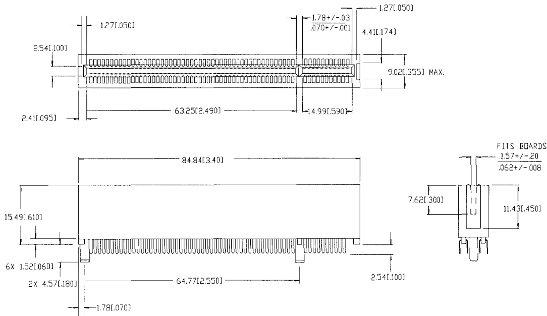
Figure 5-17: 32-bit Connector
