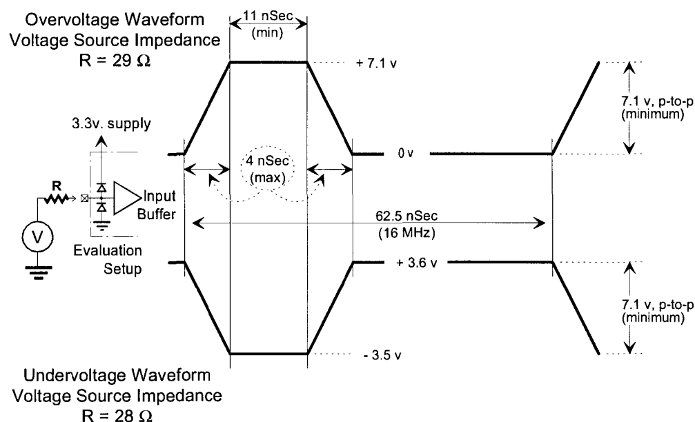
Figure 4-6: Maximum AC Waveforms for 3.3V Signaling
