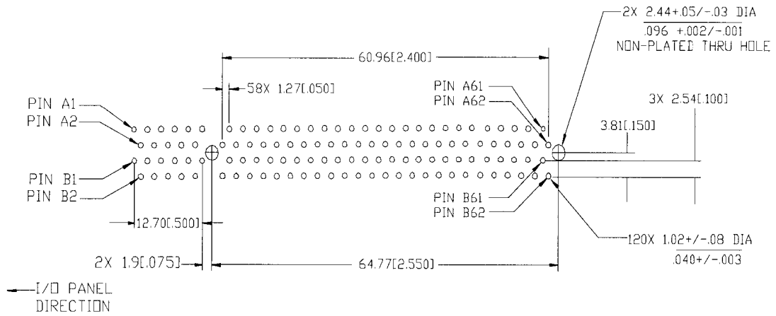
Figure 5-19: 3.3V/32-bit Connector Layout Recommendation
