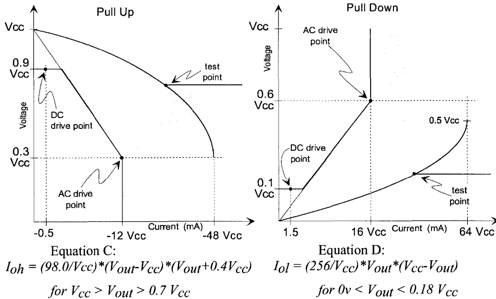
Figure 4-5: V/I Curves for 3.3V Signaling
