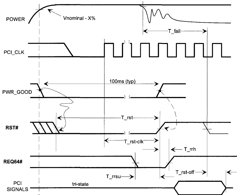
Figure 4-12: Reset Timing 35
