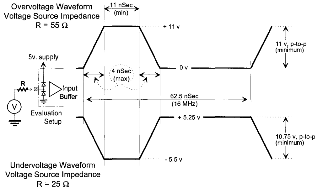
Figure 4-4: Maximum AC Waveforms for 5V Signaling
