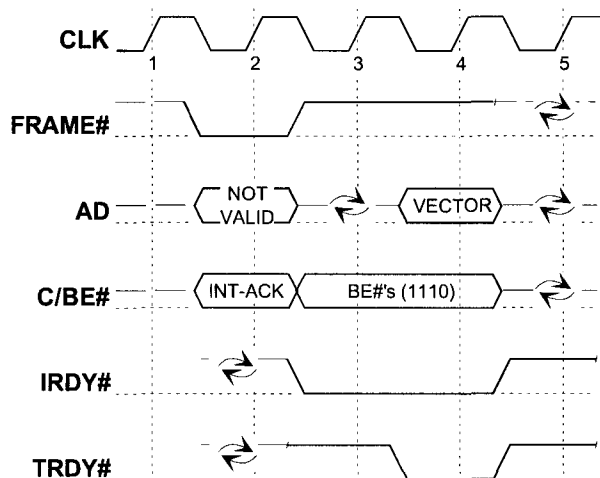
Figure 3-25: Interrupt Acknowledge Cycle
