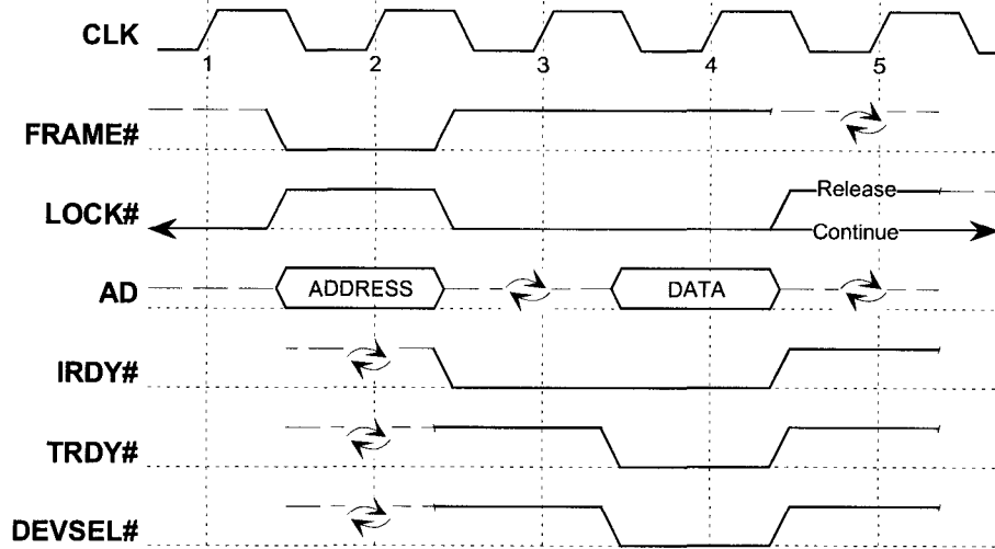
Figure 3-14: Continuing an Exclusive Access
