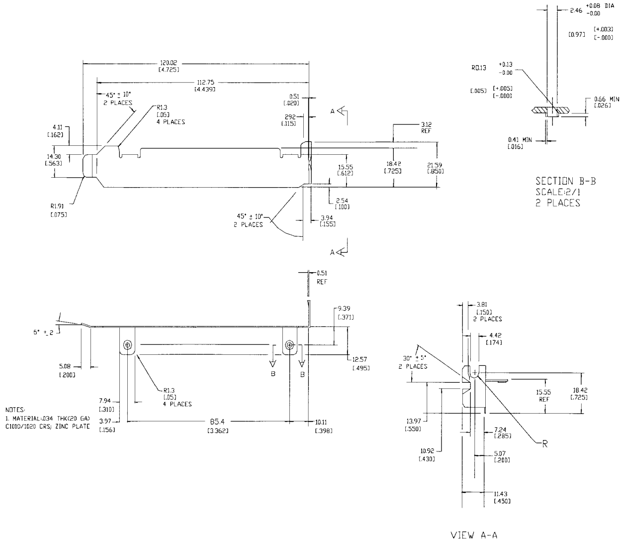
Figure 5-12: ISA Bracket
