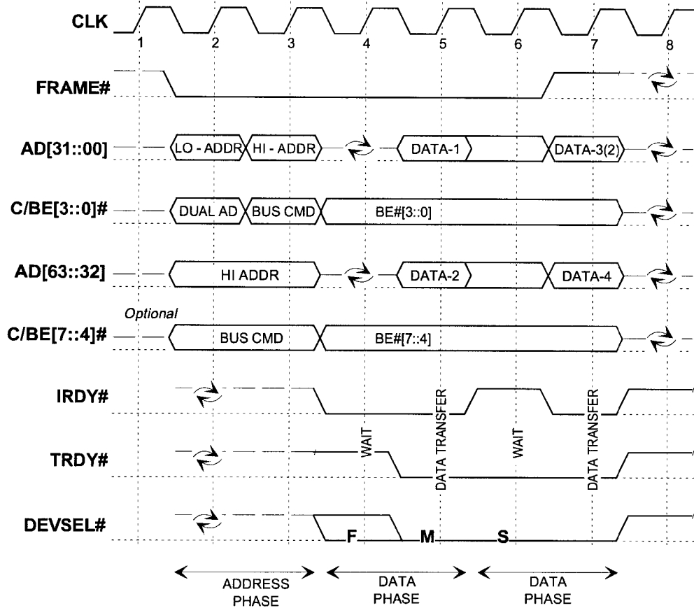
Figure 3-33. 64-Bit Dual Address Read Cycle
