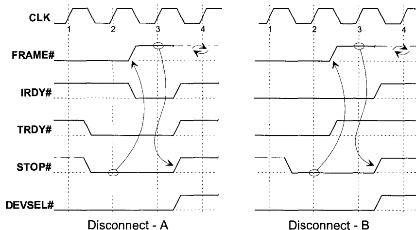
Figure 3-6: Disconnect With Data
