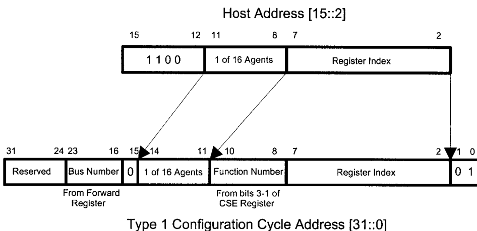
Figure 3-24: Translation to Type 1 Configuration Cycle
