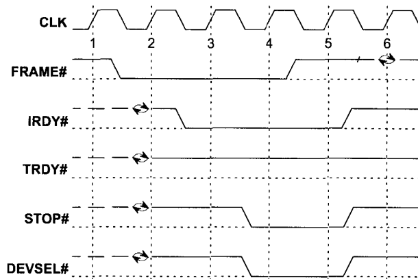
Figure 3-5: Retry
