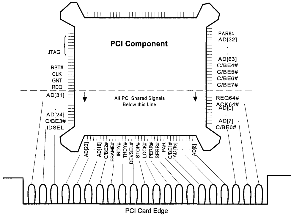
Figure 4-10: Suggested Pinout for PQFP PCI Component
