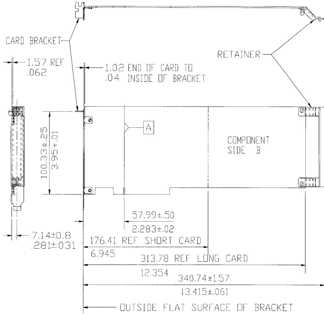
Figure 5-9: ISA Assembly (3.3V and Universal)
