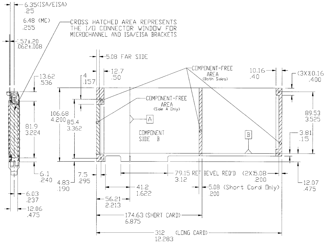
Figure 5-2: PCI Raw Card (3.3V and Universal)
