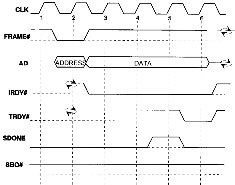
Figure 3-27: Wait States Inserted Until Snoop Completes
