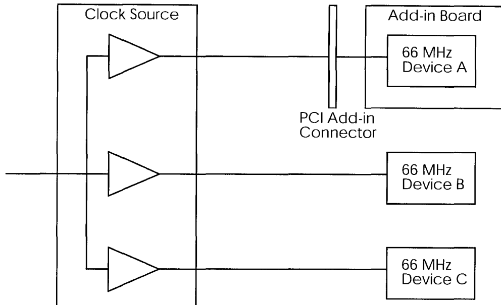
Figure 7-9: Recommended Clock Routing
