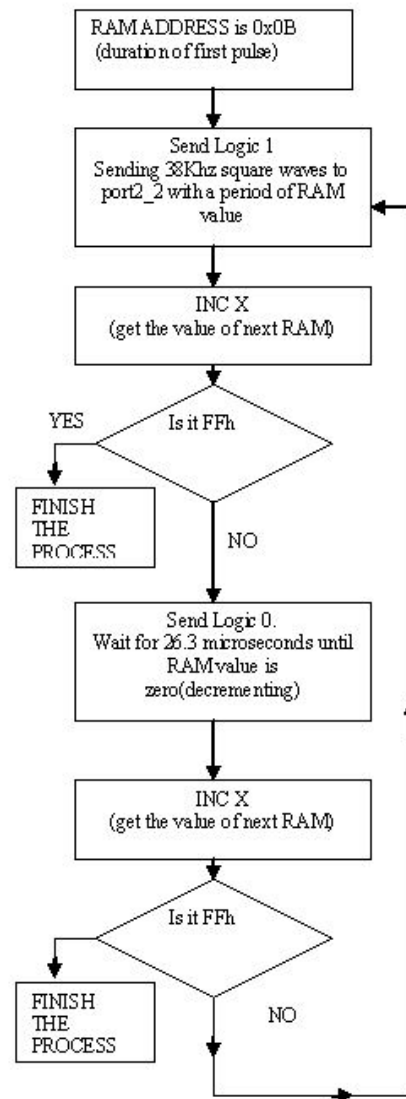
Figure 7: Process Flow
